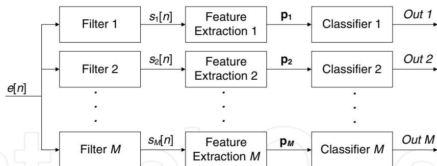
Fig. 8. Filter bank for disturbance decoupling.
