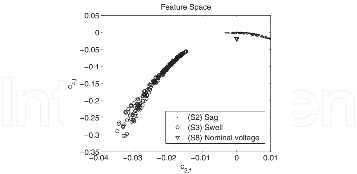
Fig. 6. Feature space for: (S2) sag, (S3) swell and (S8) nominal voltage waveform.
