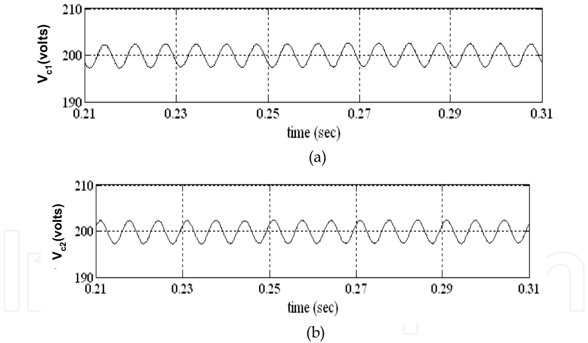
Fig. 28. DC-Bus capacitor voltages (a) Voltage across C_1 (b) Voltage across C_2
