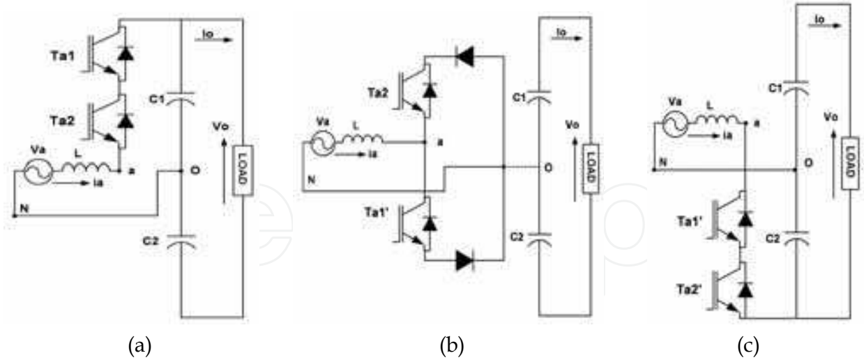
Fig. 22. Three valid operating modes for phase A of NPC rectifier (a) Mode 1 ( v_{ao} = V_o/2 ) (b) Mode 2 ( v_{ao} = 0 ) (c) Mode 3 ( v_{ao} = -V_o/2 )
