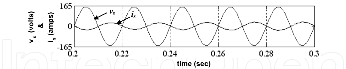
Fig. 26. Phase A voltage and line-current waveforms for inversion mode of operation
