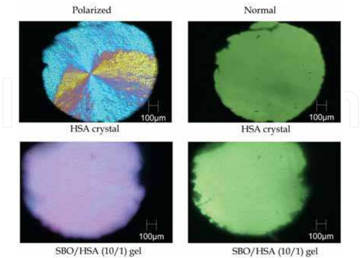
Fig. 11. Polarized and normal optical photomicrographs of HSA, SBO/HSA(10/1) gel.
