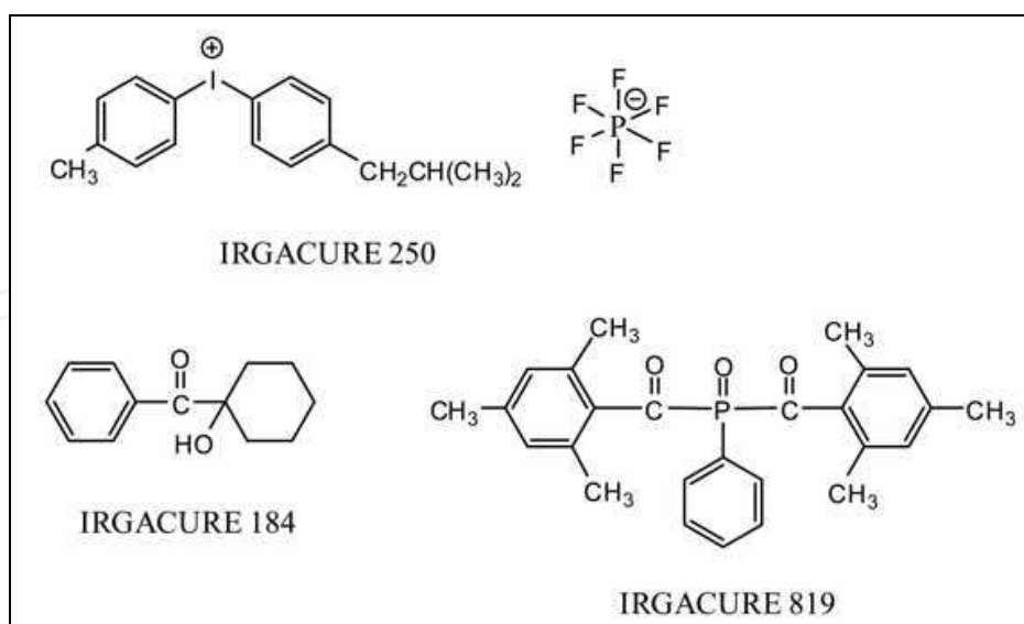
Fig. 5. Structure of photoinitiators used in this study.
