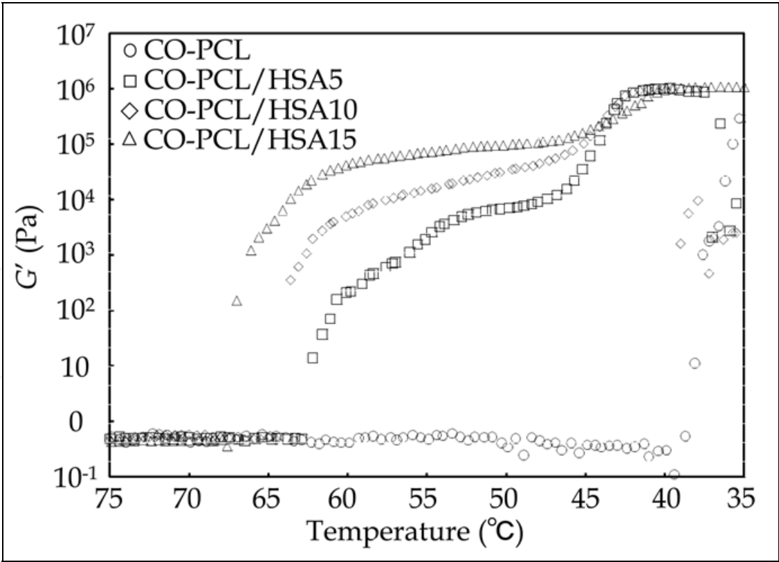
Fig. 19. Temperature dependency of G' at a cooling rate of -1\text{ }^{\circ}\text{C}/\text{min} for CO-PCL, CO-PCL/HSA5, CO-PCL/HSA10, and CO-PCL/HSA15. Reprinted from Shibata et al. (2010) with permission of John Wiley & Sons Inc.
