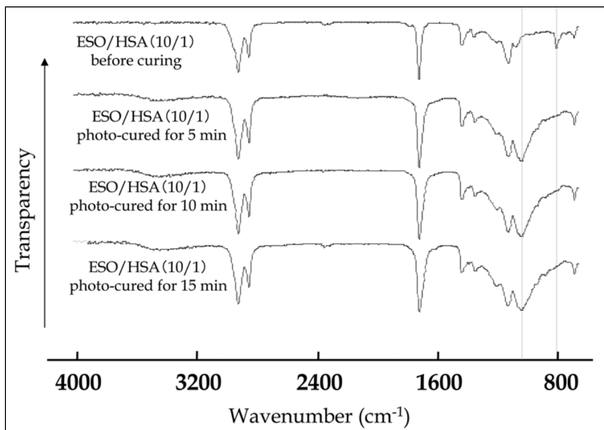
Fig. 6. FT-IR spectra of ESO/HSA(10/1) during the photo-irradiation.
