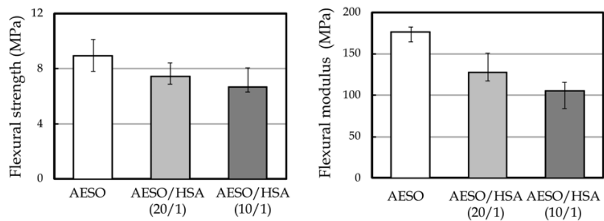
Fig. 17. Flexural properties of the photo-cured AESO/HSA composites.
