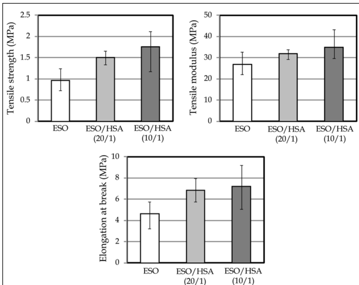
Fig. 15. Tensile properties of the photo-cured ESO/HSA nanocomposites
