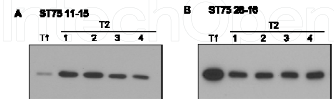
Fig. 9. Western blots showing fluctuation in transgene expression levels between generations. A. Equal amounts (1µg) of seed protein from a T 1 parent and four T 2 progeny were examined to reveal an increase in mSEB expression. B. Equal amounts (1µg) of seed protein from a T 1 parent and four T 2 progeny were examined and reveal a decrease in mSEB expression.
