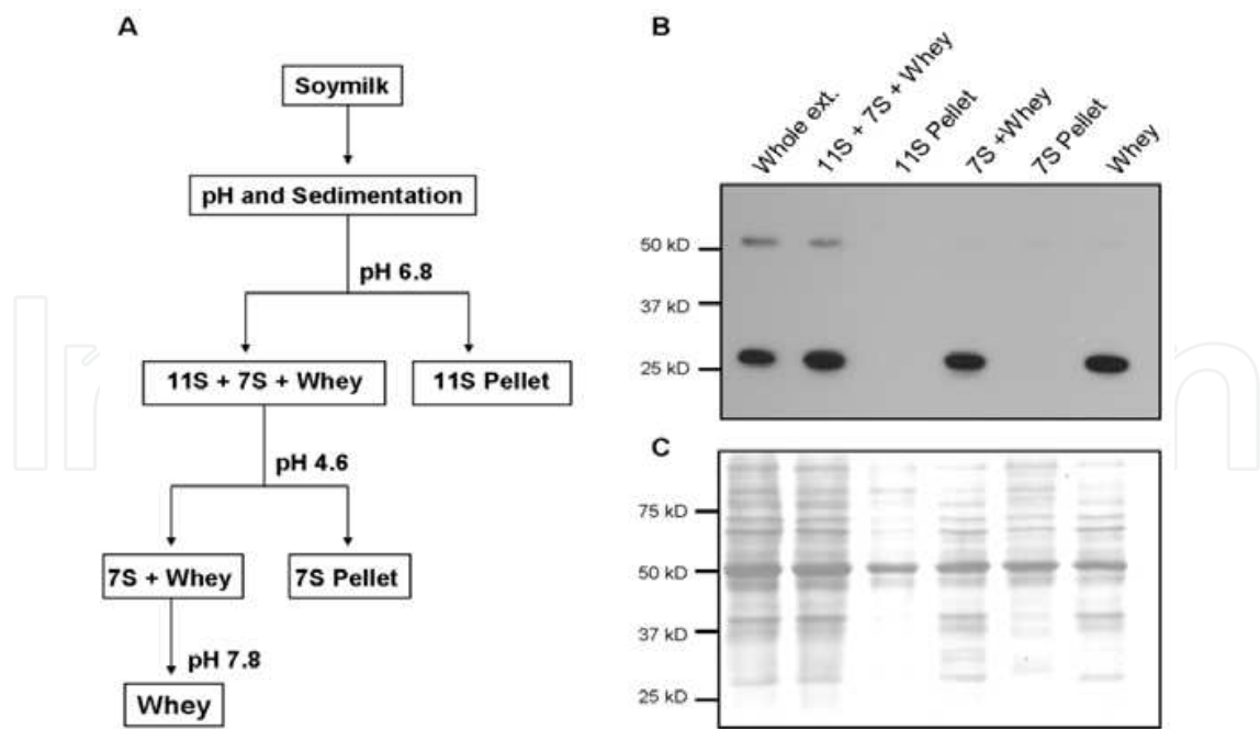
Fig. 10. Partial purification of mSEB using isoelectric fractionation. A. Schematic of soybean protein families that precipitate at various pH. B. Western blot (top panel) and coomassie-stained membrane (bottom panel) of soymilk protein (20ug) following isoelectric fractionation.
