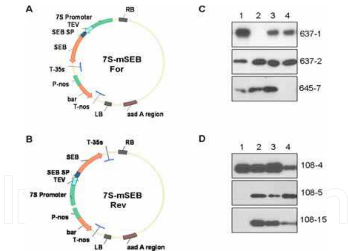
Fig. 8. Gene cassettes in opposing orientation and western analysis of T 1 progeny from events transformed with both orientations . A. The 7S-mSEB gene cassette in the forward orientation containing the 7S seed-specific promoter, TEV leader, native SEB signal peptide, mSEB gene, and 35S terminator elements. B. The 7S-mSEB gene cassette in the reverse orientation containing the same elements as the forward version. C. Western blot analysis showing protein expression of seeds from a transformation event with the cassette in the forward orientation. D. Protein expression from a transformation event with the cassette in the reverse orientation.
