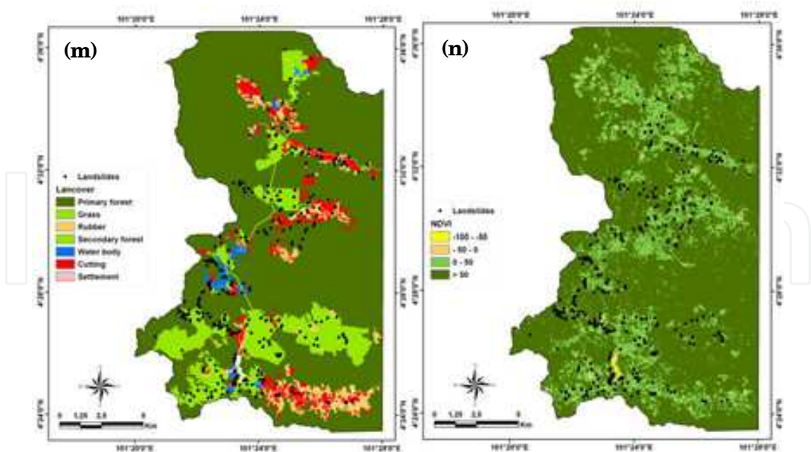
Fig. 2. Input data layers (a) Slope; (b) Aspect; (c) Curvature; (d) Stream power index (spi); (e) Distance from drainage; (f) Flow length; (g) Flow accumulation; (h) Topographic wetness index; (i) Distance to road; (j) Lithology; (k) Distance to the fault lines; (l) Soil types; (m) Land cover; and (n) Vegetation index (NDVI)
