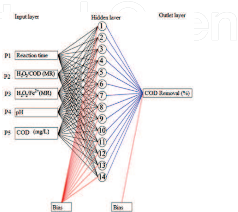
Fig. 4. Artificial neural network optimized structure (Elmolla et al., 2010)
