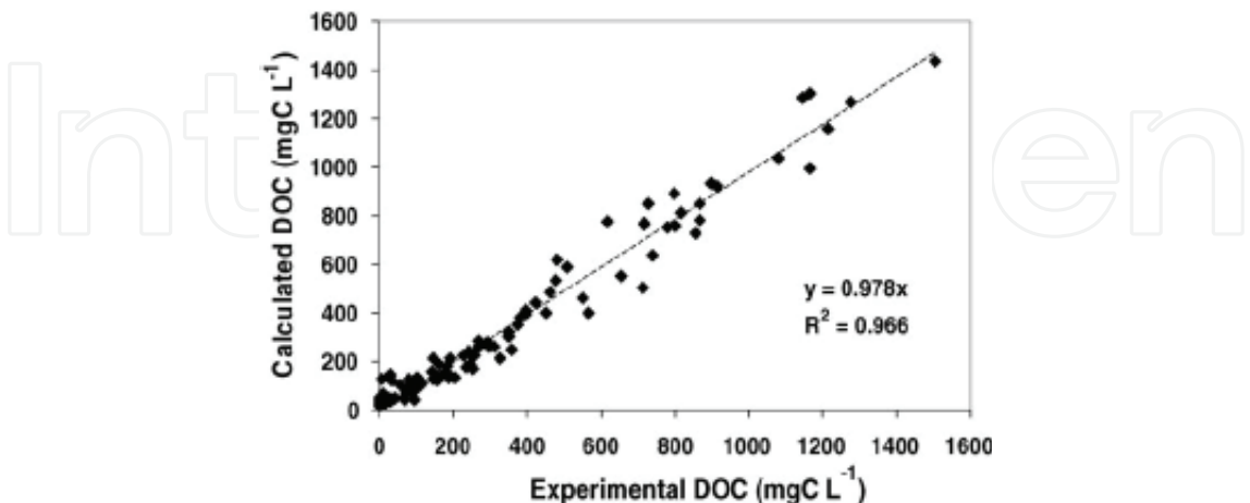
Fig. 8. Comparison between calculated and experimental DOC (Giroto et al., 2006)
