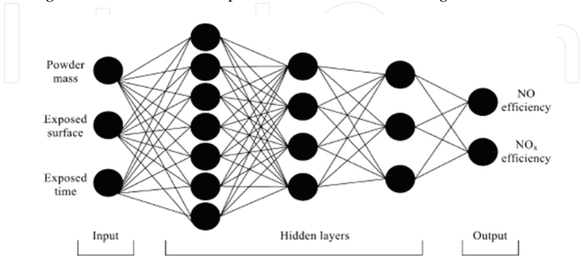
Fig. 14. Artificial neural network optimized structure (Toma et al., 2004)
