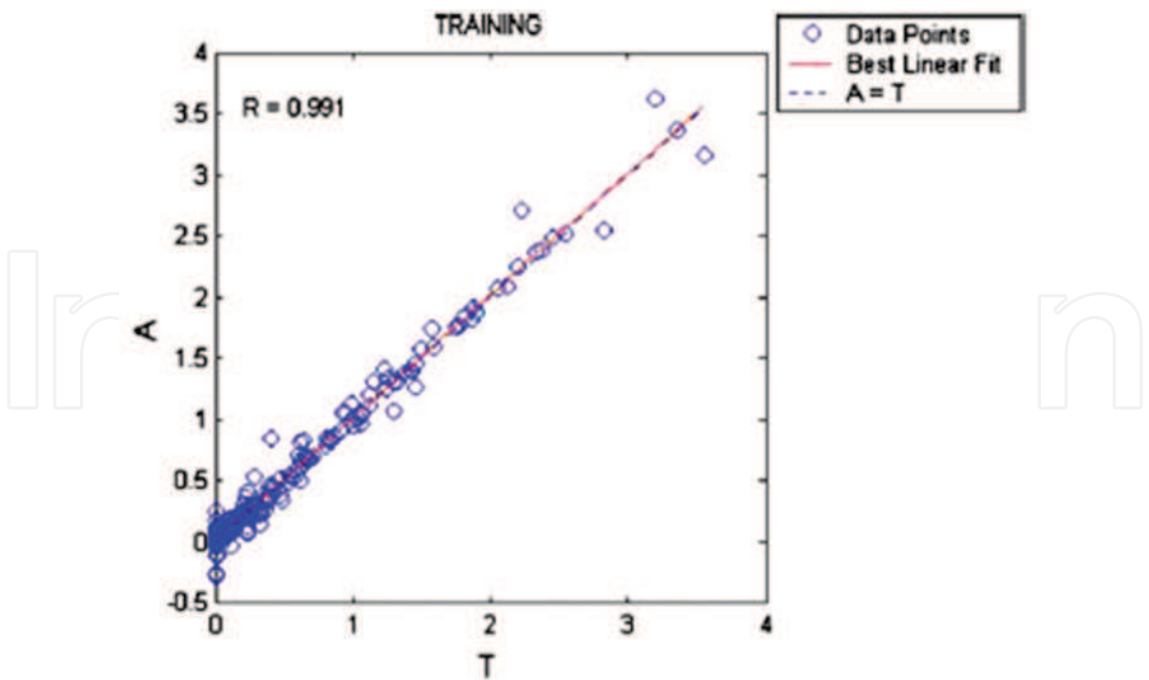
Fig. 11. Comparison between predicted and measured absorbance (Guimarães et al., 2008)
