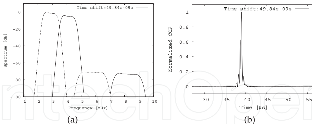
Fig. 24. Received signals of proposed coded THI when \xi = 0.05\mu\text{s} . (a) Frequency spectrum and (b) CCF.
