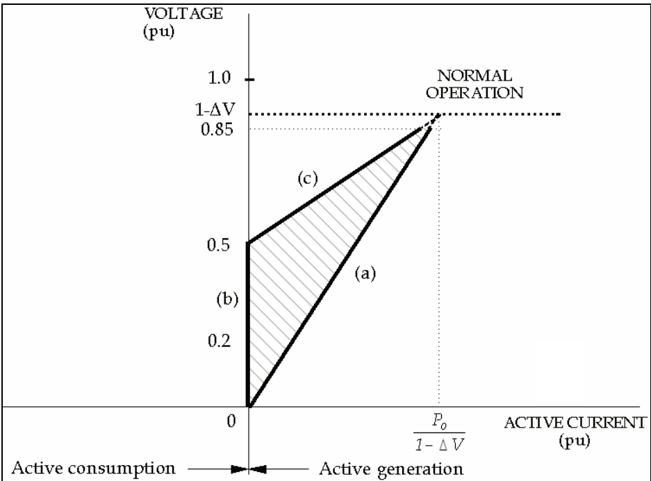
Fig. 8. Active current limits in unitary values during the voltage dip Active current values according to the O.P. 12.2 must be within the area showed in fig.8. Limits of the active current described in fig.8 are mathematically expressed in unitary values as:
