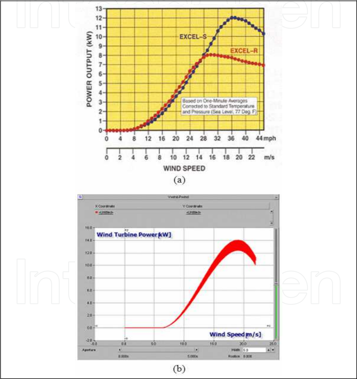
Fig. 5. The compare of characteristic curves (a) The characteristic curve of wind turbine output (b) The output characteristics of simulation model of wind turbine
