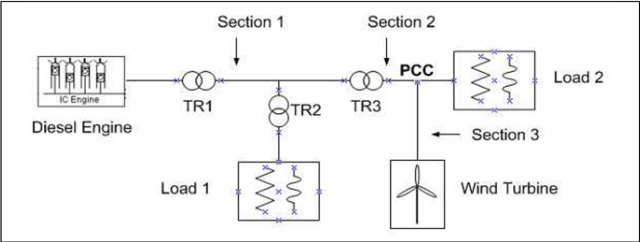
Fig. 2. Outline of power supply system in Sapsido A more detailed explanation of the components is shown in Table 1. All contents of Table 1, except for the generator, are applied in modeling and only one 300[kVA] generator is modeled for convenience of modeling. Impedance of the line attains its scale value at the point indicated as the section in Fig. 2, just as indicated in Table 2 according to kinds and length of cable. It applies an almost similar value even though there is little difference according to each manufacturing company.
