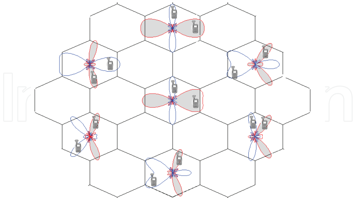
Fig. 2. Network Topology
