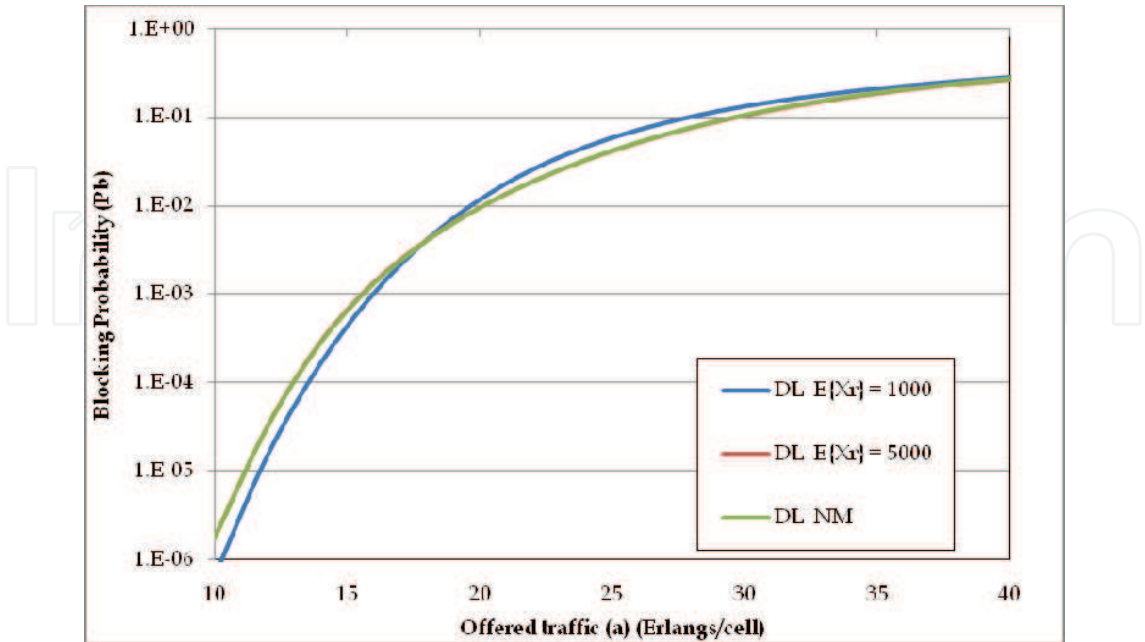
Fig. 5. Blocking Probability for a system with Duplicate at Last Policy. No link unreliability is considered.
