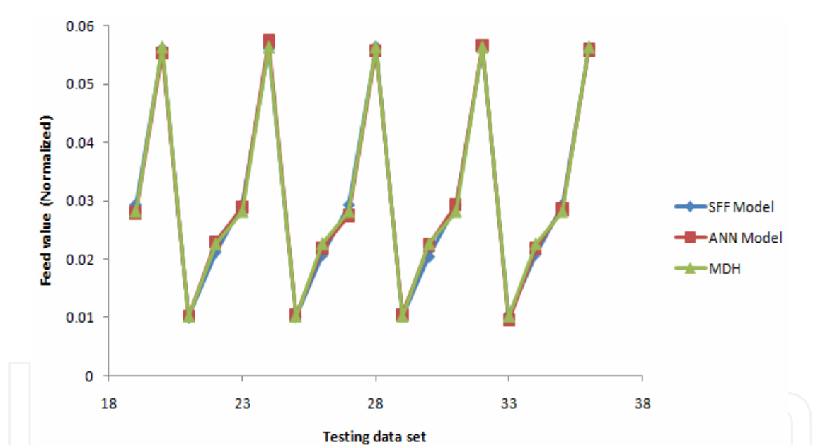
Fig. 21. Comparison of feed values between SFF, ANN and MDH
