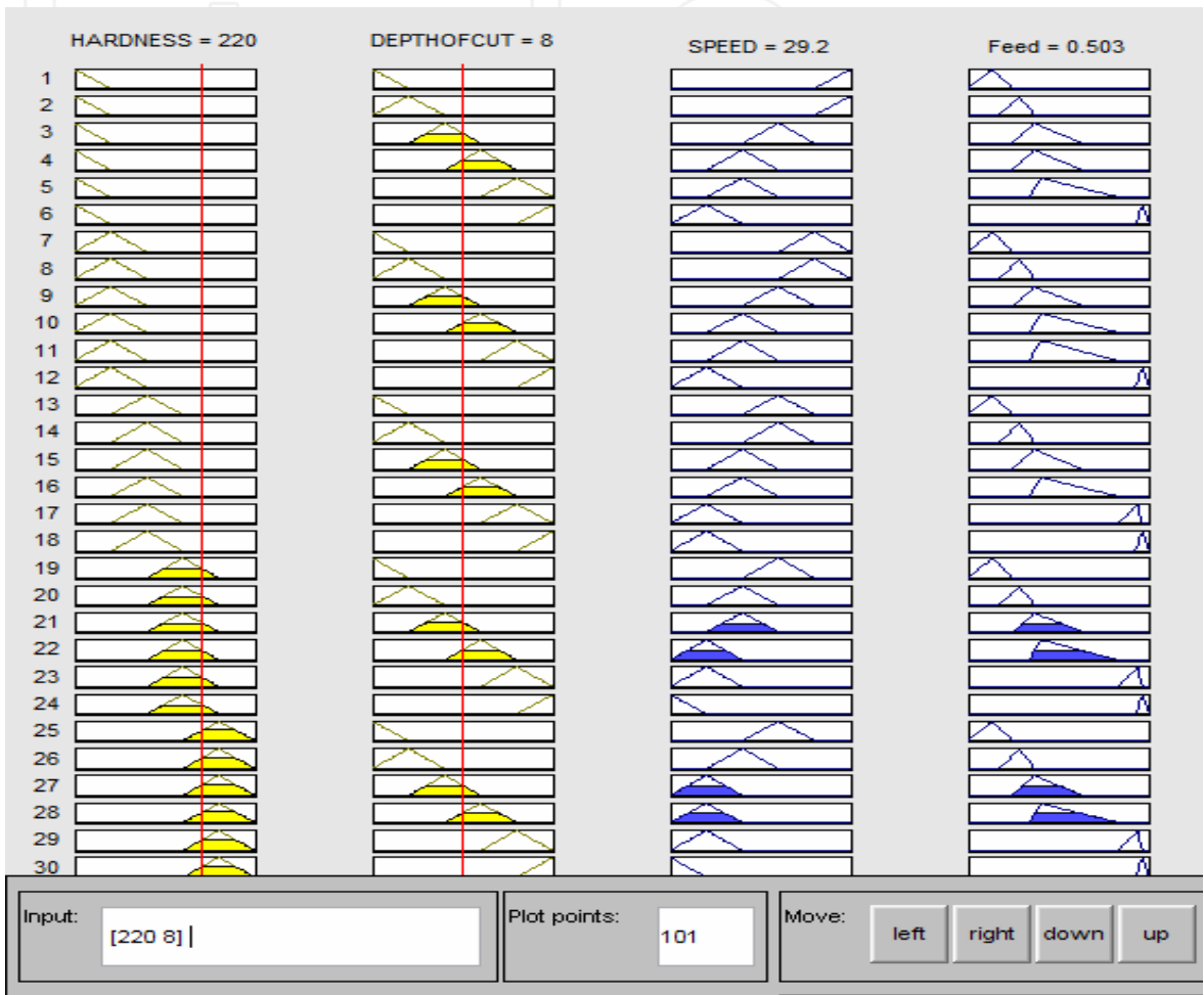
Fig. 12. User-friendly viewer for the SFF model (from MATLAB) The viewer shown in Fig.12 is used to generate the input-output samples. The values are tabulated in Tables 4 and 5. The tables show the validation of the predicted values of cutting speed and feed found by the SFF model with the Machining Data Handbook. Seventy two different values of wrought carbon steel hardness from (85-275) BHN and depth of cut from (1-16) mm were selected for this comparison. For demonstration purpose two tool types are used: high speed steel (HSS) tool and uncoated brazed carbide (Carbide) tool. The SFF model is applied to obtain the outputs speed and feed and the values are then compared. The absolute error percentage is calculated for each value and the mean absolute error percentages are obtained for the 36 samples. The mean error percentage is almost 7% for speed and 4% for feed when using high speed steel tool and for carbide tool is almost 8% for speed and 7% for feed (Table 6). In order to get better results, the density of the selected samples can be increased.
