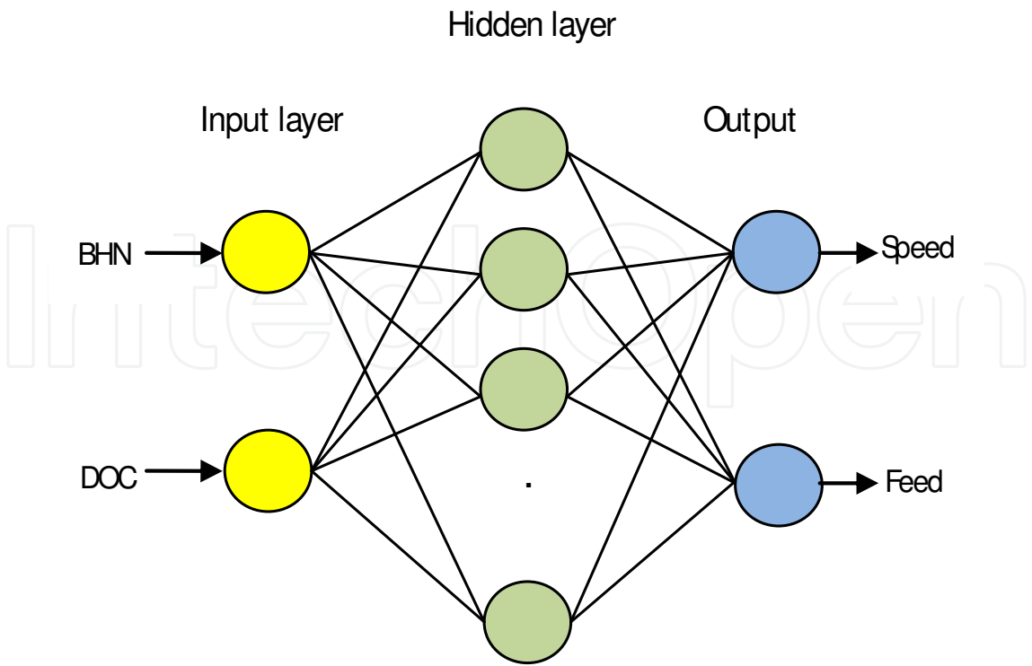
Fig. 11. Neural network structure for machining parameters
