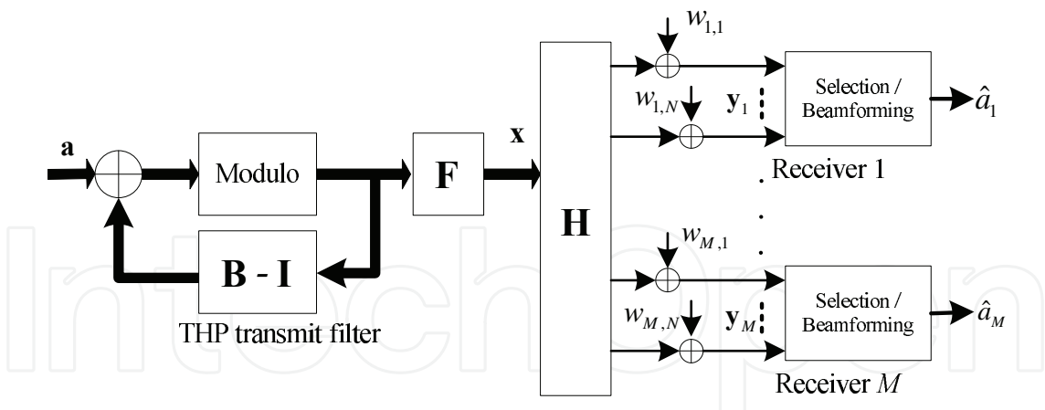
Fig. 1. Block diagram of ZF-THP in multiuser MIMO downlink system.
