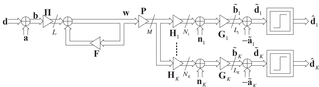
Fig. 3. Equivalent linear representation of THP in Fig. 2.
