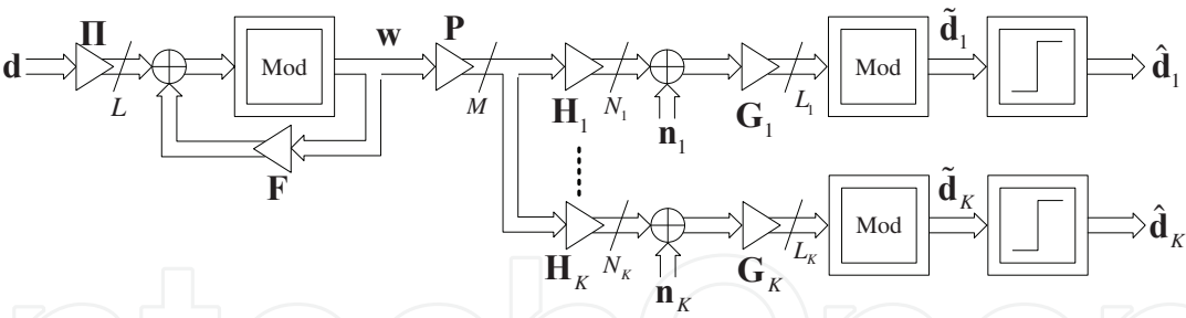
Fig. 2. Block diagram of MMSE-THP in multiuser MIMO downlink system.
