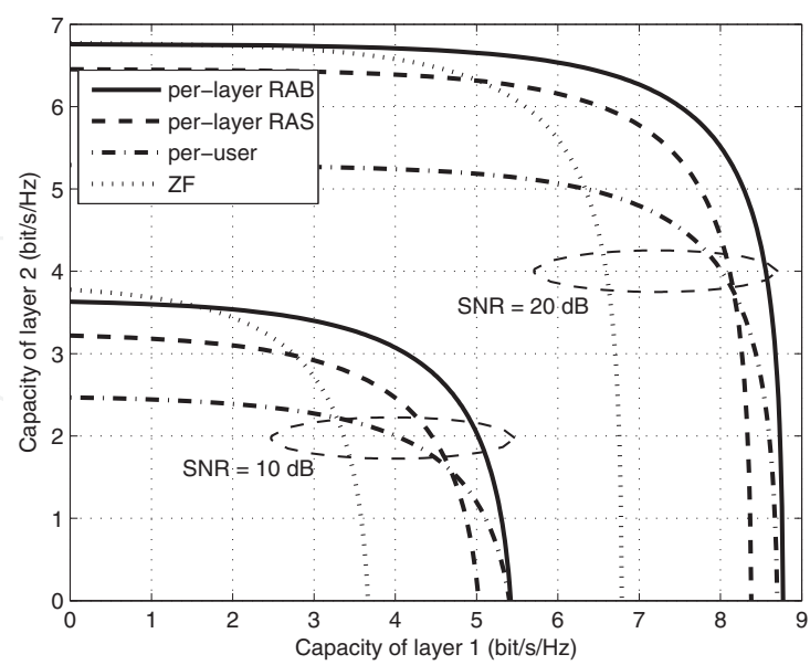
Fig. 6. The rate regions in (2 \times 2) \times 2 systems.
