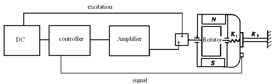
Fig. 11. Active control shock absorber functional diagram
