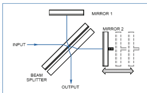
Fig. 2. Schematic description of a Michelson interferogram.
