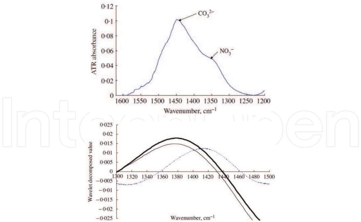
Fig. 7. Overlapping bands of nitrate and carbonate in ATR spectra of calcareous soils (Top frame) and the wavelet decomposed values at scale 2 (dashed, attributed to carbonate) and at scale 3 (attributed to nitrate, 14ppm and 120ppm N-NO 3 ) (Bottom frame). Reproduced from Jahn et al. (2006).
