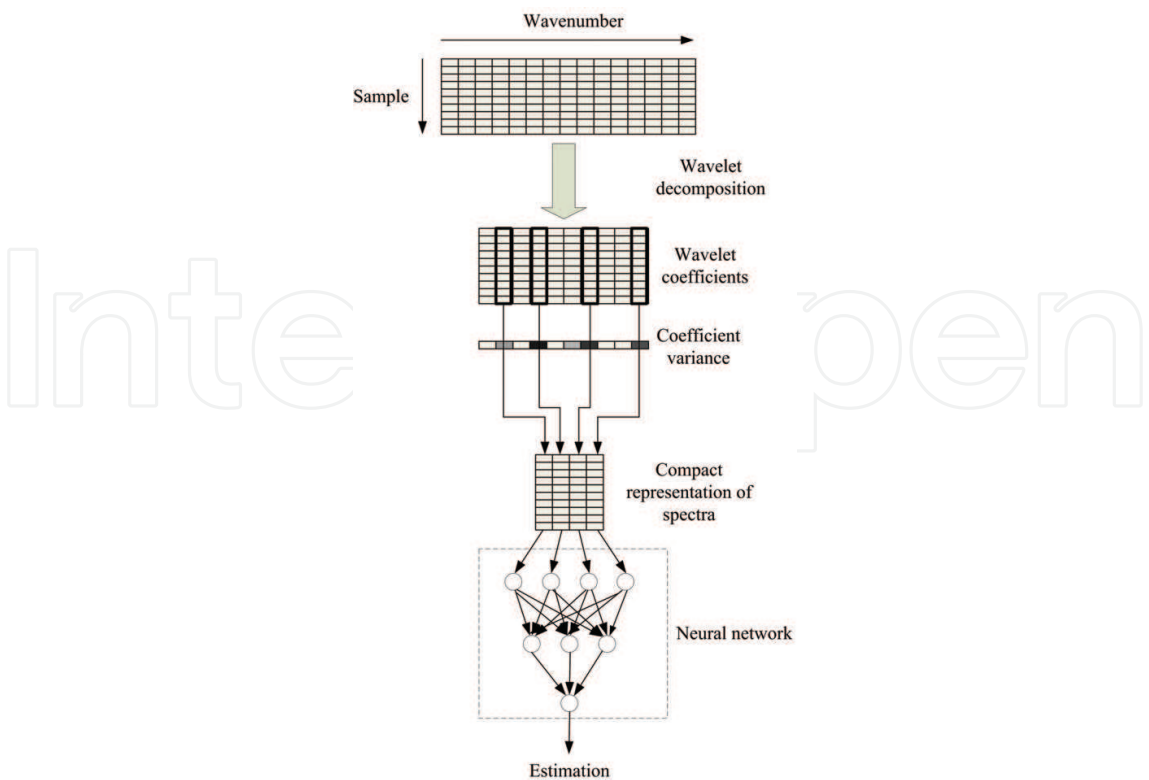
Fig. 6. Schematic representation of a prediction model combining wavelet decomposition of the spectra and a neural network
