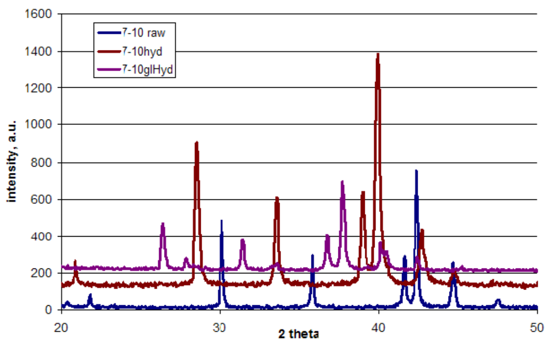
Fig. 11. XRD plot of raw (7-10raw), hydrogenated pure 7-10 (7-10H) and hydrogenated alloy 7-10 with glass phase (7-10gl-H)
