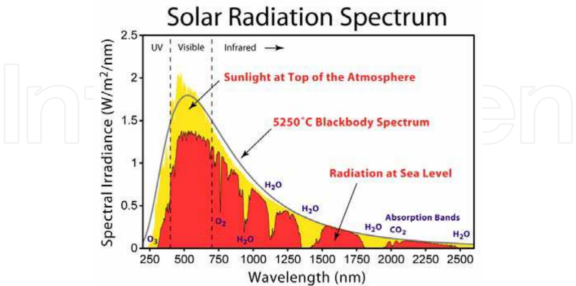
Fig. 2.1. Solar irradiance spectrum above atmosphere and at surface Image created by Robert A. Rohde / Global Warming Art ( http://www.globalwarmingart.com/wiki/File:Solar_Spectrum_png )
