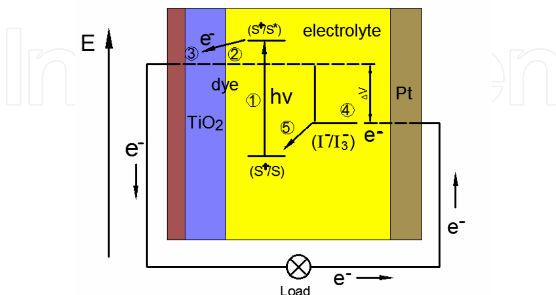
Fig. 4.14. Principle of operation and energy level scheme of the dye-sensitized nanocrystalline solar cell. Potential are referred to the standard calomel electrode (SCE) (Hagfeldt & Grätzel, 1995). The redox system is iodide/triiodide-based redox electrolyte. S stands for sensitizer; S^* , electronically excited sensitizer; S^+ , oxidized sensitizer
