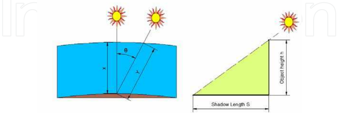
Fig. 2.2. AM measurement The measurement of AM is in Figure 2.2. Here h is the object height, s is the shadow length. From the geometry, the AM can be calculated:
