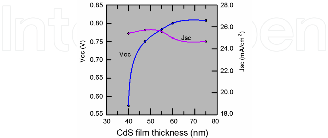
Fig. 4.8. The V_{oc} and J_{sc} as a function of CdS film thickness Data comes from (Kumazawa et al., 1997)
