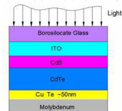
Fig. 4.9. Schematic of device configuration on Mo foil substrate (Singh et al., 1999)
