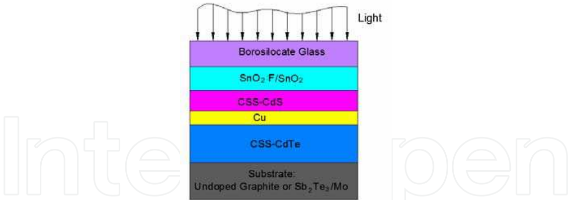
Fig. 4.7. Cu was incorporated into the device prior to the CdTe deposition (Barri et al, 2005)
