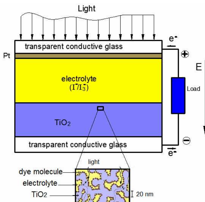
Fig. 4.13. A schematic diagram of structure and components of a DSSC solar cell
