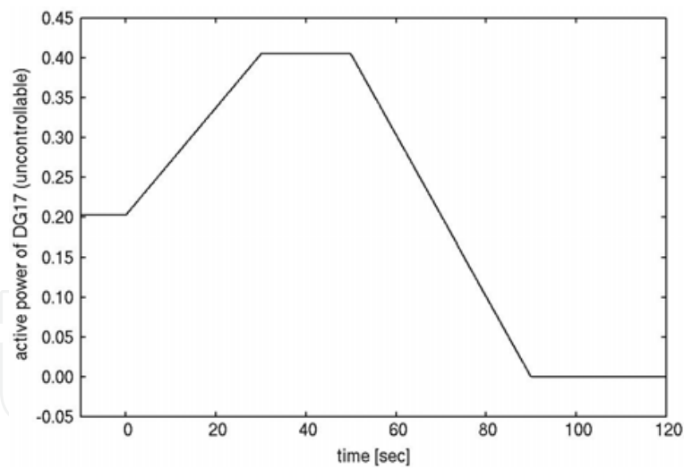
Fig. 22. Active power change of DG17.
