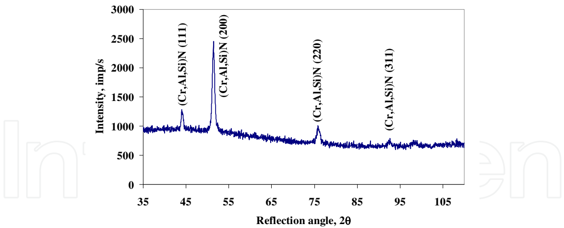
Fig. 6. GAXRD spectra of the CrAlSiN coating at glancing incidence angle \alpha=2^\circ .
