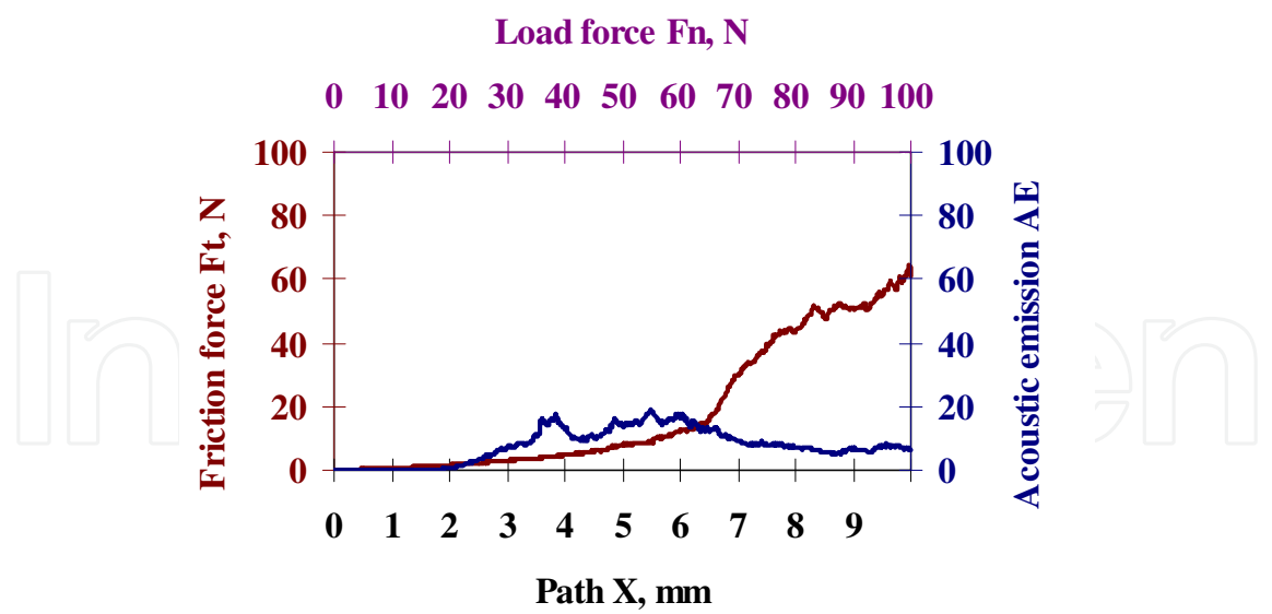
Fig. 11. Diagram of the dependence of the acoustic emission (AE) and friction force F_t on the load for the X40CrMoV5-1 steel with the TiAlSiN coating.
