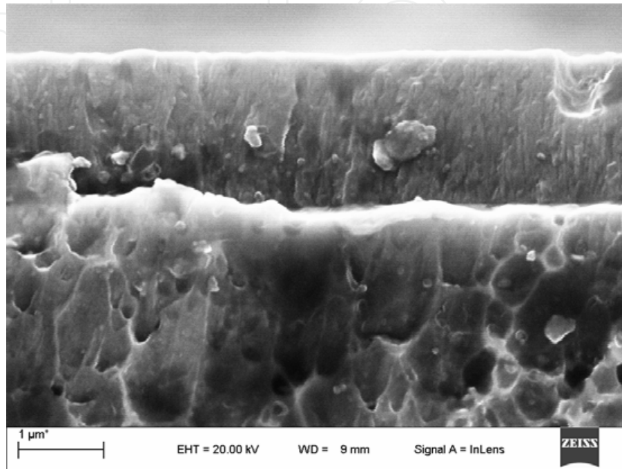
Fig. 1. Fracture of the TiAlSiN coating deposited onto the X40CrMoV5-1 steel substrate.
