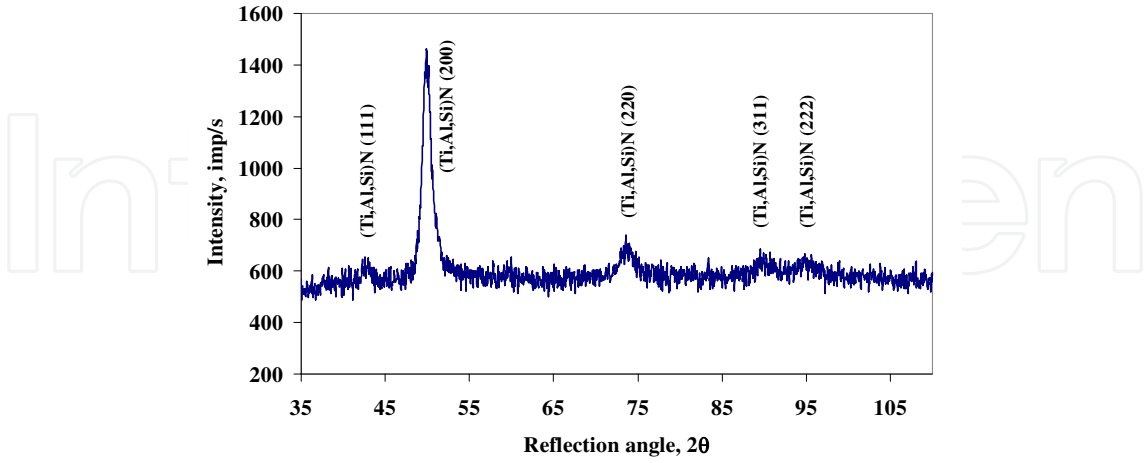
Fig. 8. GAXRD spectra of the TiAlSiN coating at glancing incidence angle \alpha=2^\circ .
