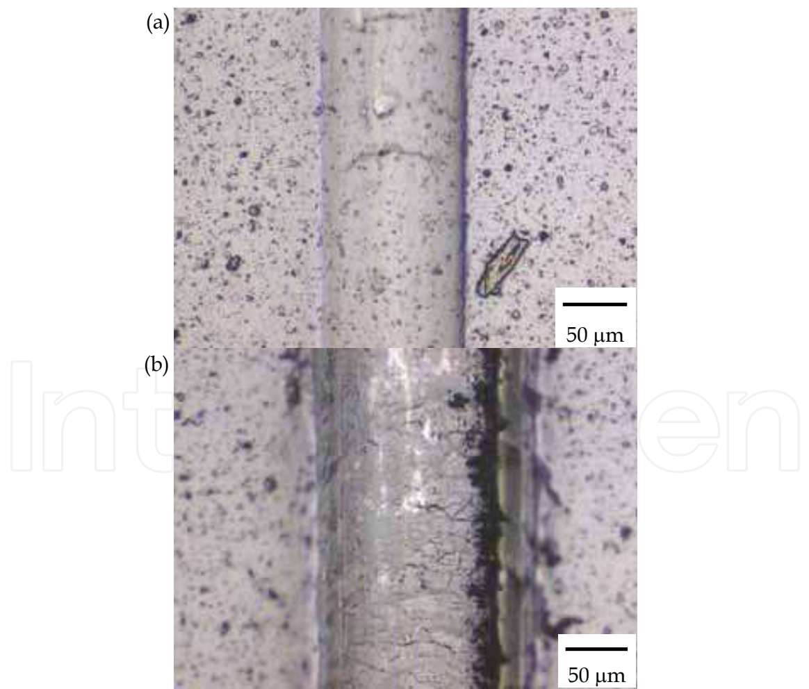
Fig. 12. Scratch failure pictures of the AlTiCrN coating on X40CrMoV5-1 steel substrate at: (a) L_{C1} , (b) L_{C2} .
