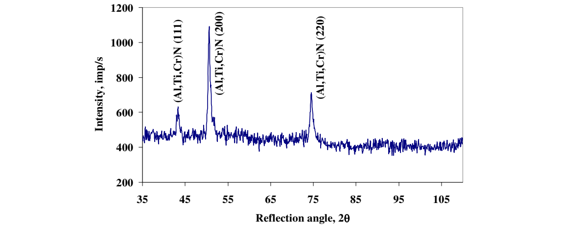
Fig. 7. GAXRD spectra of the AlTiCrN coating at glancing incidence angle \alpha=2^\circ .
