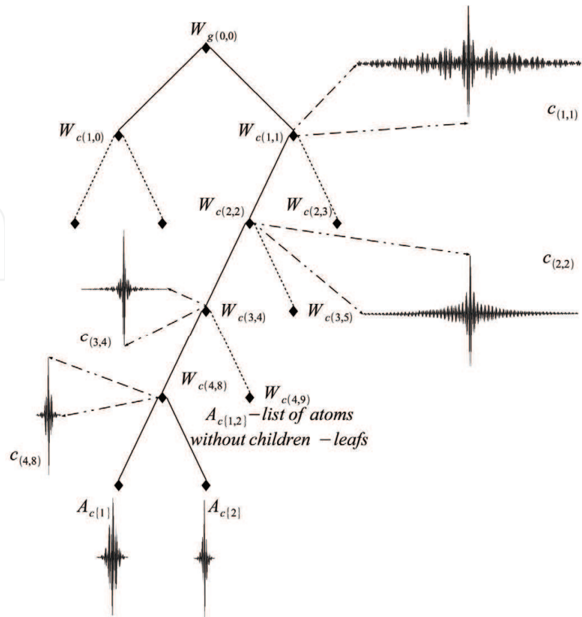
Fig. 1. Example dictionary structure
