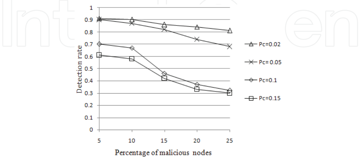
Fig. 15. Detection ratio of malicious nodes
