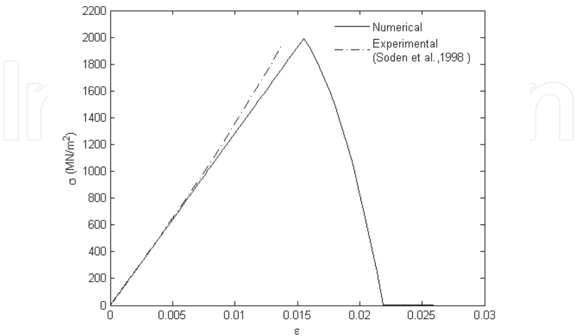
Fig. 1. Stress vs strain relationship in fibre direction for the tension test.
