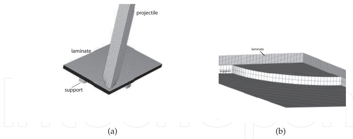
Fig. 4. Initial setup: (a) A quarter of the real configuration is used in the numerical tests thanks to the symmetry. (b) A closer snapshot of the laminate and the support.
