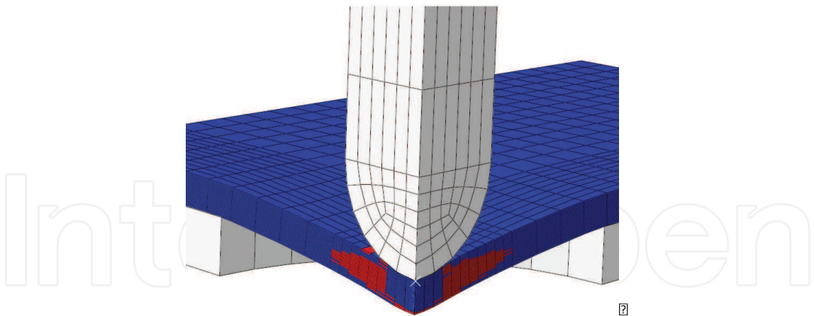
Fig. 6. Matrix cracking pattern using a classical failure criterium based on stress components. The elements in red fulfilled the criterium which means that they are not withstanding loads any longer.
