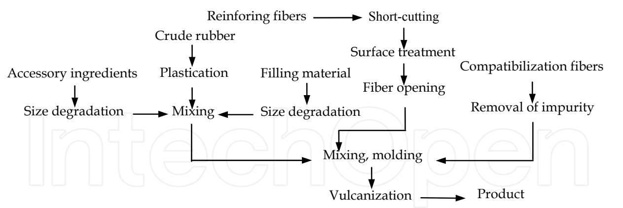
Fig. 1. A molding process of NASC
