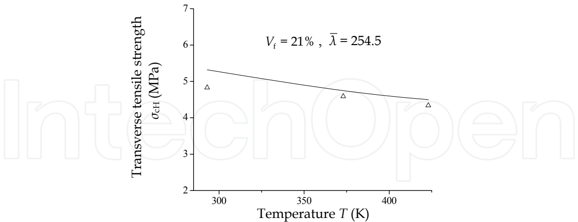
Fig. 22. Effect of temperature on transverse tensile strength
