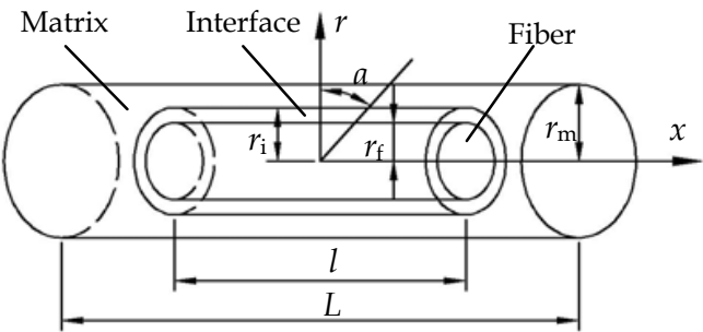
Fig. 12. A micromechanical model of NASC The stress transfer procedure can be seen in Fig. 13.
