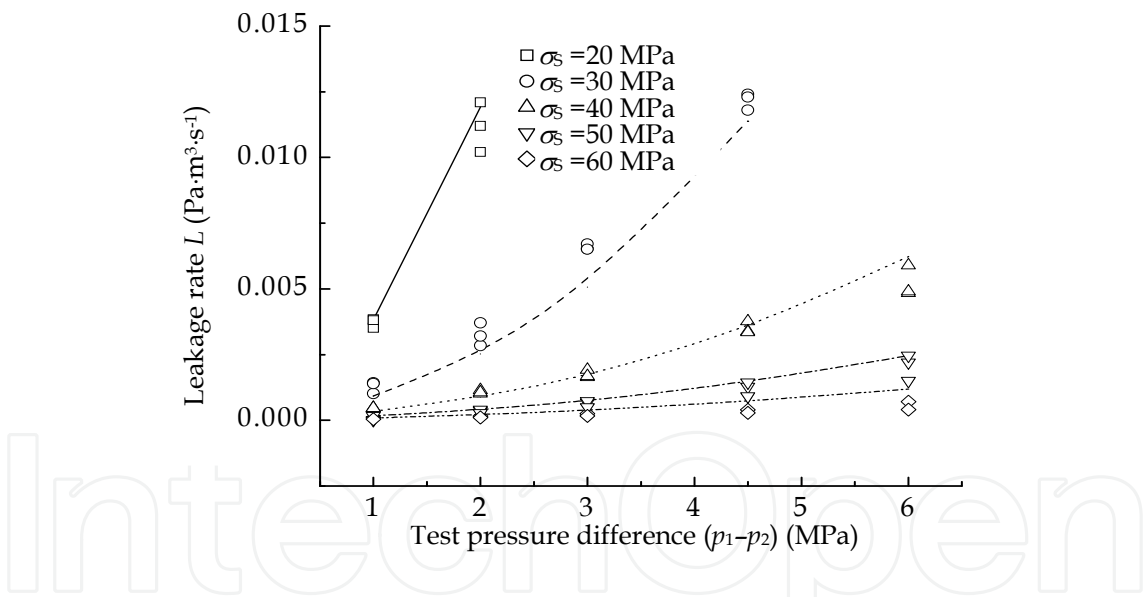
Fig. 26. Relationship between leakage rate and test pressure difference under different seating stresses
