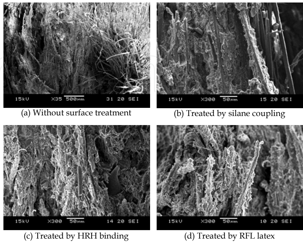
Fig. 5. SEM photos of transverse tensile fracture sections of aramid fiber reinforced NASC
