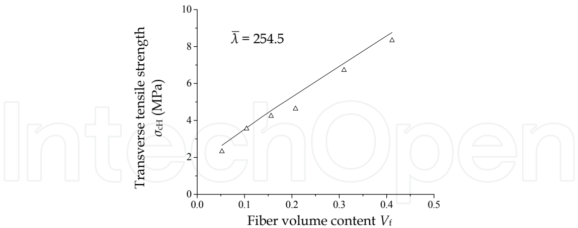
Fig. 21. Relationship between transverse tensile strength and fiber volume content
