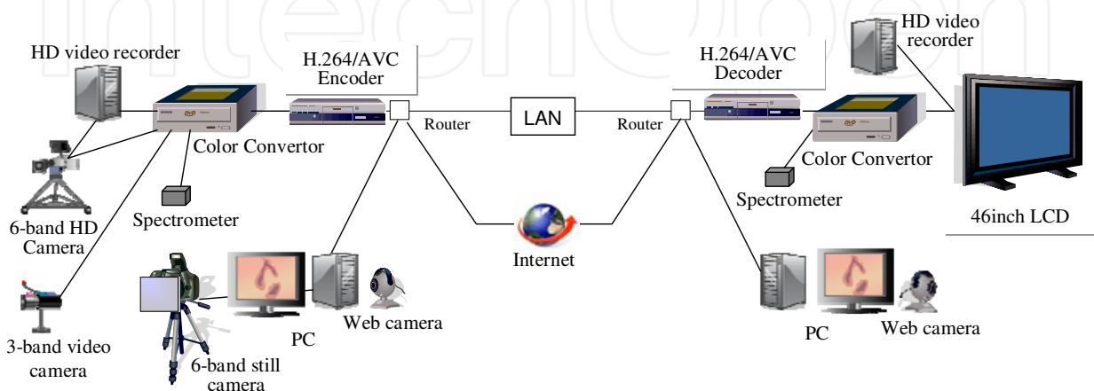
Fig. 3. System overview used in the experiments.
