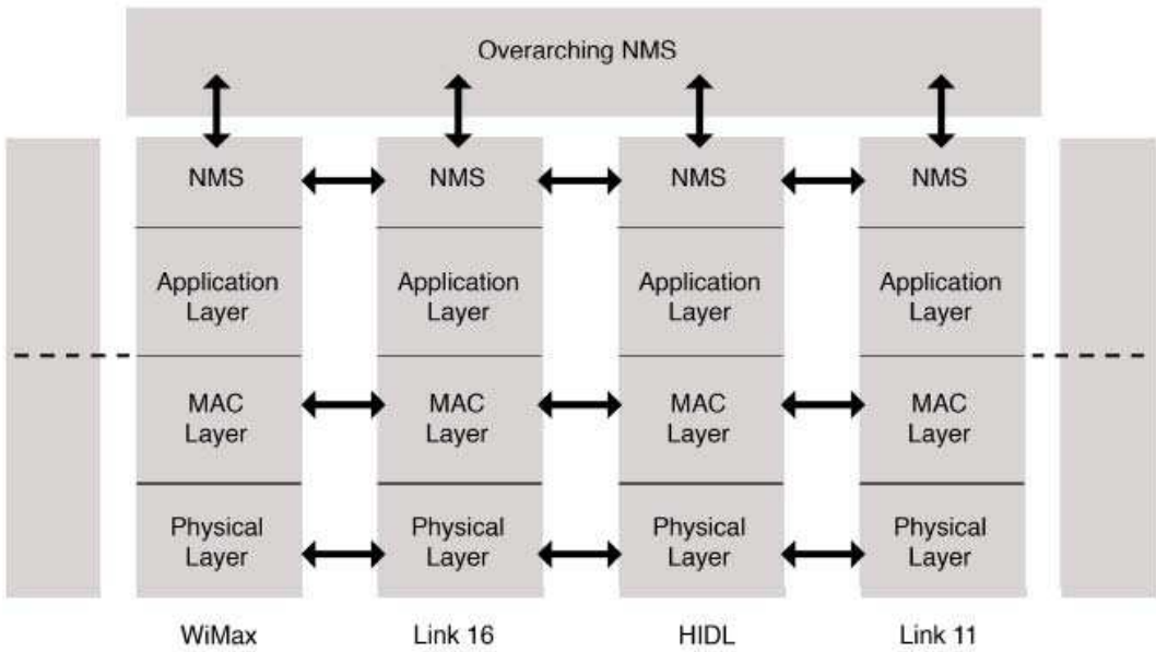
Fig. 12. Overarching Network Management System
