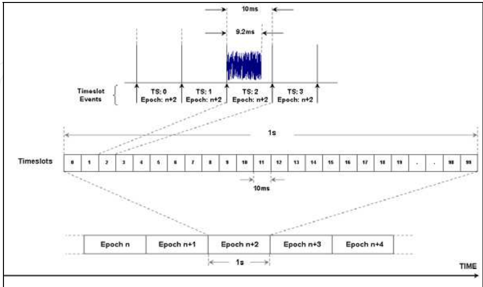
Fig. 2. The HIDL Time Architecture (Tarter, et.al., 2008)
