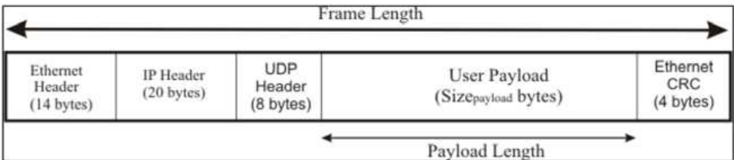
Fig. 3. The HIDL Packet Format
