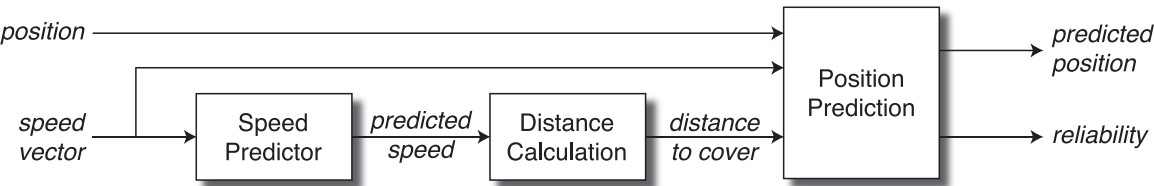
Fig. 1. Algorithm Outline
