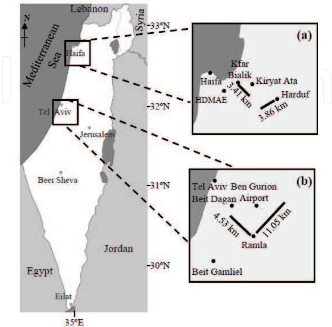
Fig. 1. The examined regions (taken from David et al., 2009). 1(a) North Israel: Two microwave links are presented (marked as lines) in front of Kiryat Ata, Haifa bay (where the humidity gauge is located). The first link (3.86 km long) is located on two hills, its transmitter and receiver are found at heights of 265 and 233 m Above Sea Level (ASL). The distance from the surface station to a point located in the middle of this wireless link is 7.5 km. The transmitting and receiving units of the second radio link (3.41 km) are situated 25 and 41 m ASL while the surface station- link distance is 3 km in this case. The Kiryat Ata surface station is situated 45 m ASL. 1(b) Central Israel: The two microwave links in front of Ben-Gurion airport meteorological station (humidity gauge's location). The distance from the surface station to a point located in the middle of the 4.53 km link is 6.5 km. This link's transmitter and receiver are located at heights of 95 and 63 m ASL. The longer link (11.05 km) is located 5 km from the surface station while its transmitting and receiving units are situated 116 and 98 m ASL. The airport surface station is situated at 41 m ASL
