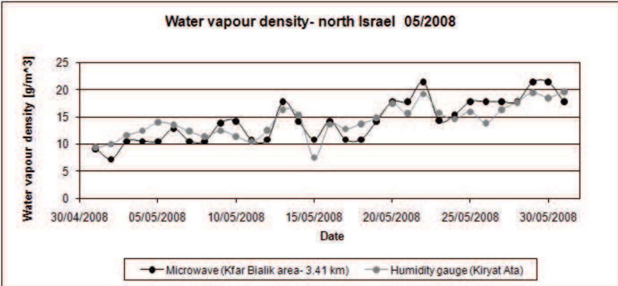
Fig. 2(b). Northern Israel - The humidity measurements were made, by the 3.41 km microwave link, during May 2008. The correlation between the two measurements is 0.87 with RMSD of 2 [g/ m³]. Link's frequency: 22.05 GHz
