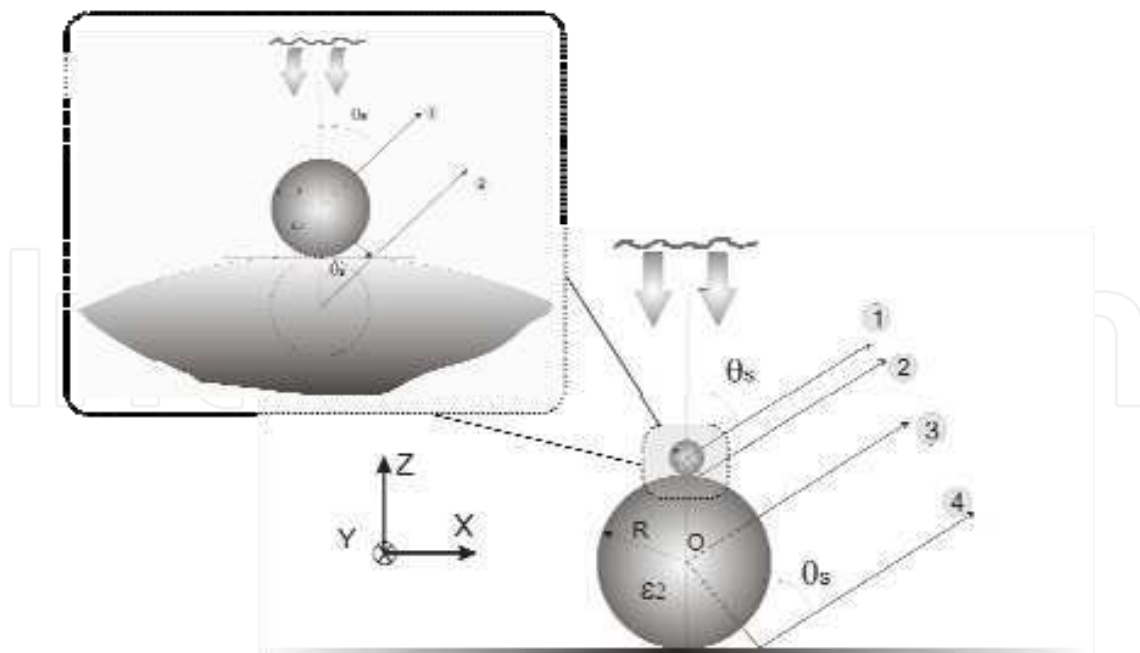
Fig. 13. Multiple interaction model for two structures illuminated at normal incidence. Inset shows the flat substrate approximation and image theory applied to the defect.
