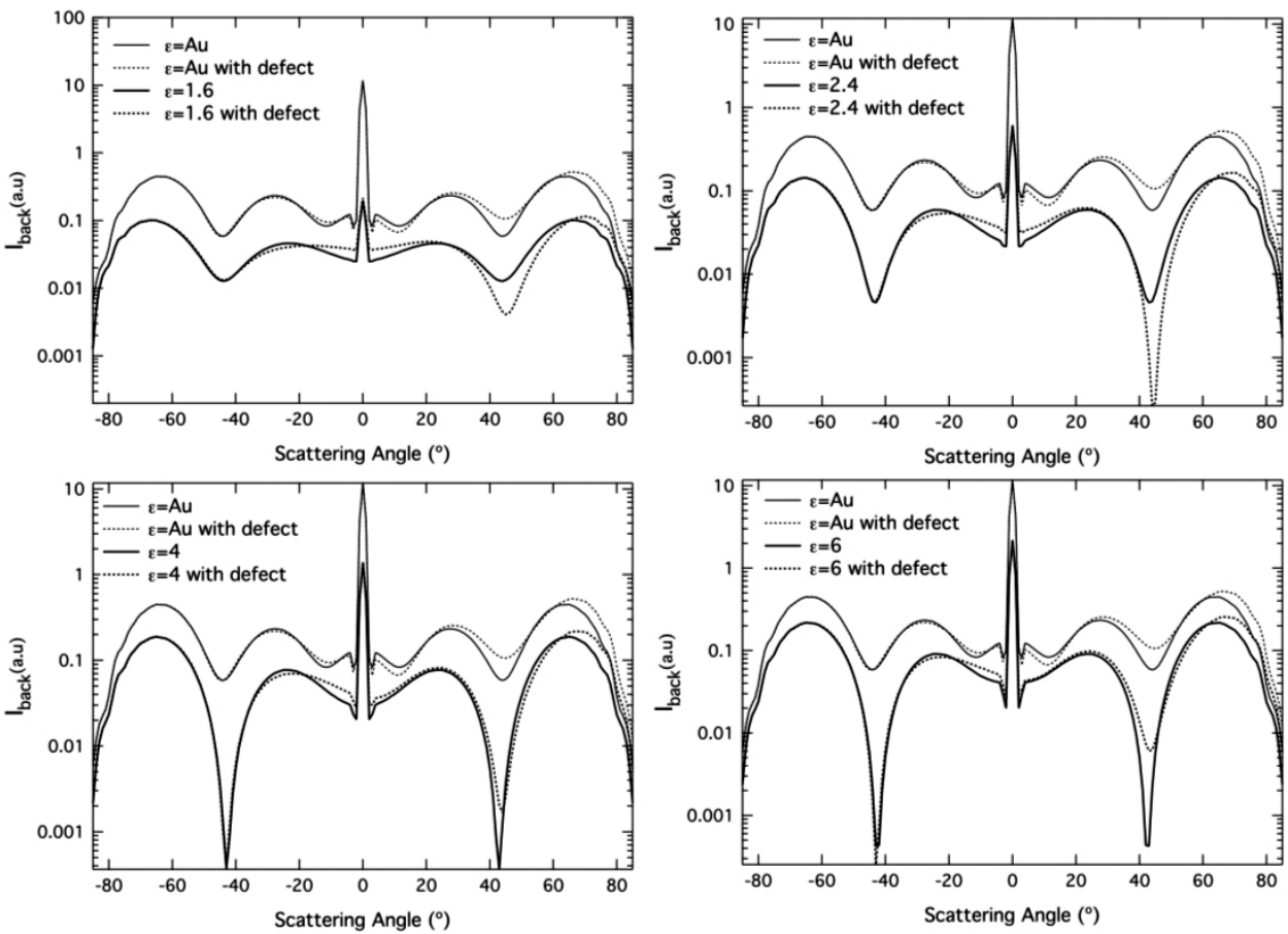
Fig. 8. Backscattering patterns for a defect on a cylinder placed on a substrate for different substrate optical properties ( \epsilon ). The defect and cylinder are made of gold and of size d = 0.1\lambda and D = \lambda respectively.
