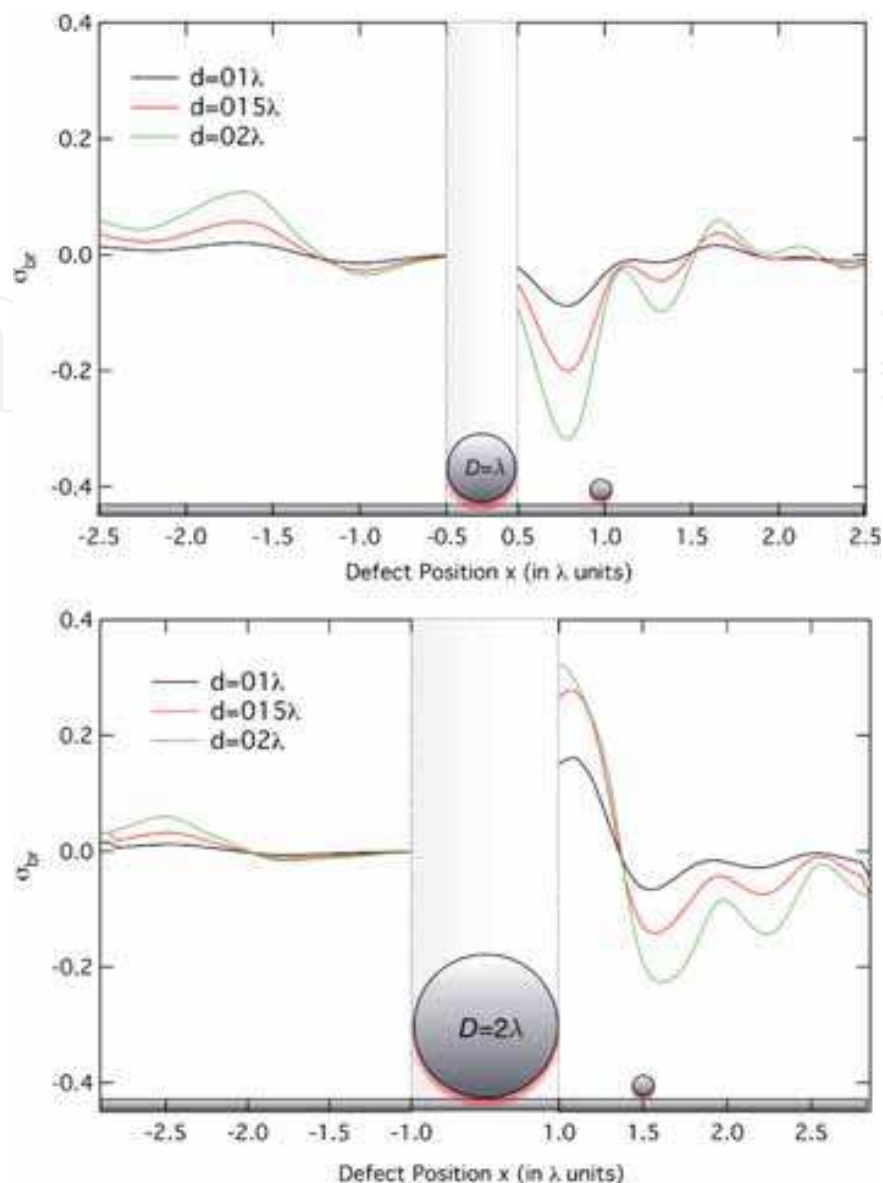
Fig. 6. \sigma_{br} for two different cylinders sizes, D = \lambda, 2\lambda and three defect sizes d = 0.1\lambda, 0.15\lambda and 0.2\lambda . Defect position x ranges from 0.5\lambda to 3\lambda from the center of the Cylinder [Albella et al. , 2007].
