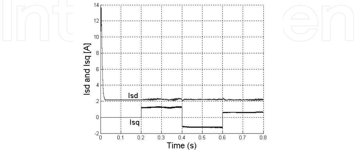
Fig. 11. Stator currents in stator flux reference frame.
