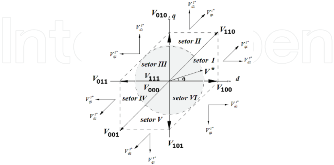
Fig. 6. Space Vectors spatial disposition.
