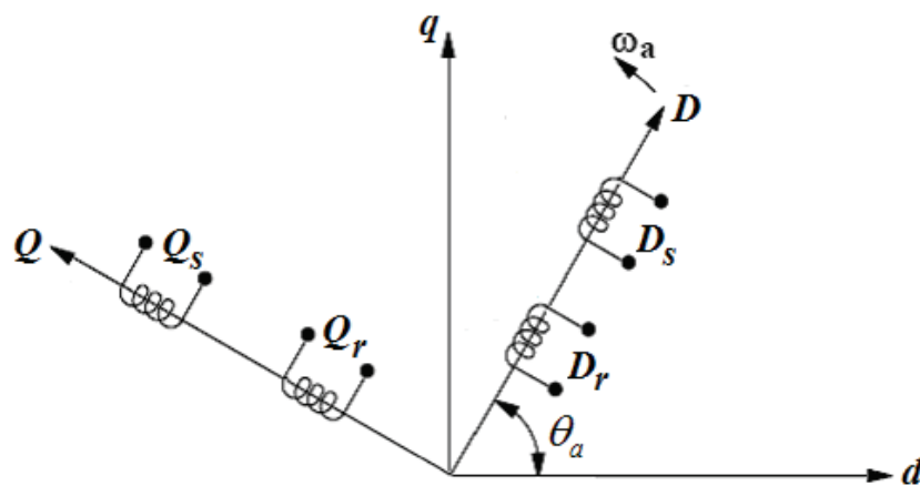
Fig. 3. Revolving reference frame.
