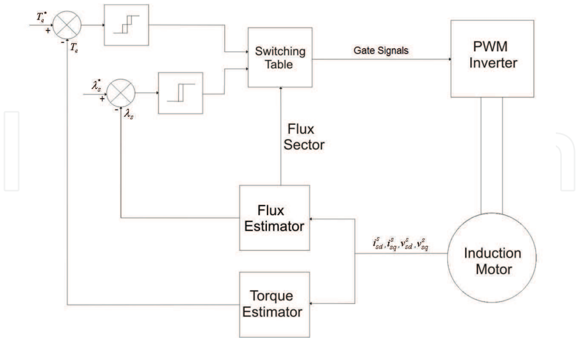
Fig. 4. Block diagram of the basic DTC scheme.
