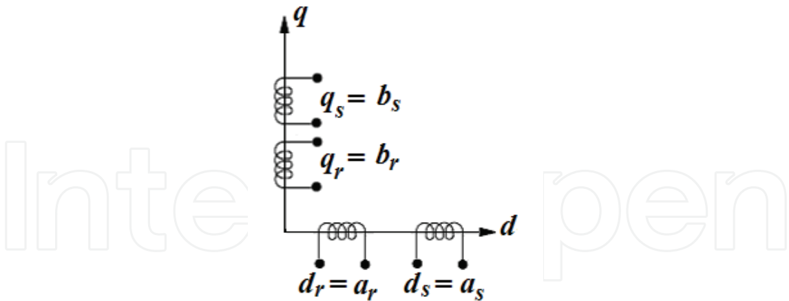
Fig. 2. Stationary reference frame ( d-q ).
