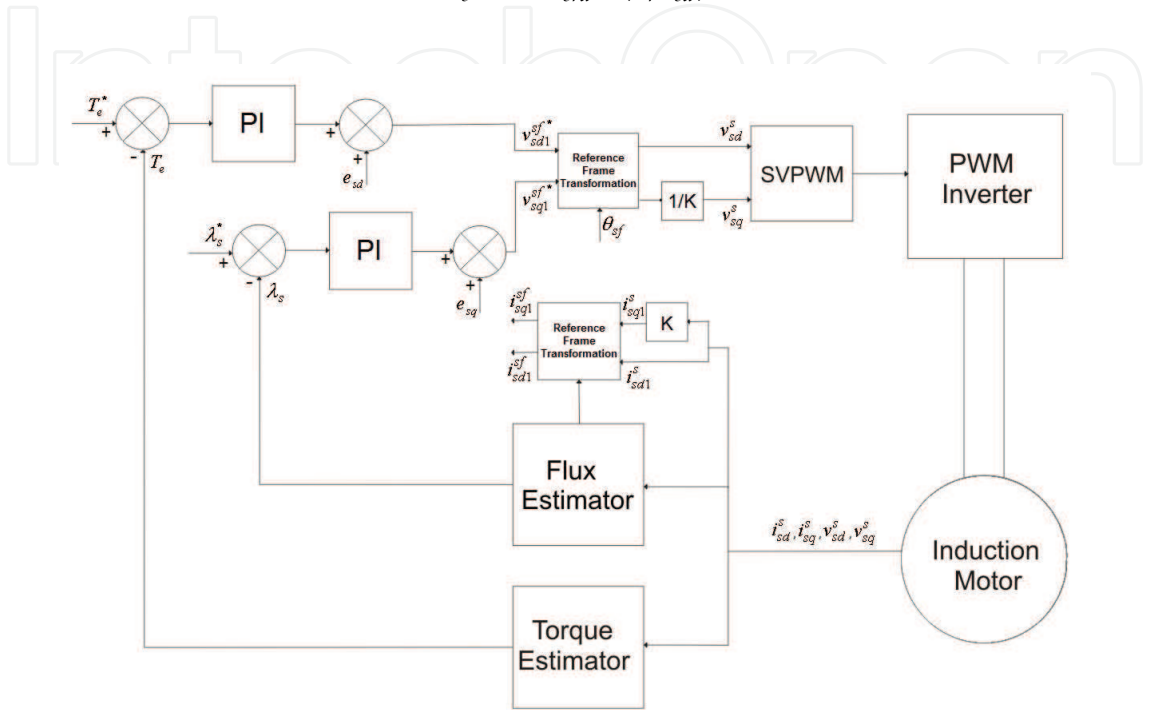
Fig. 7. SVPWM-DTC proposed scheme.
