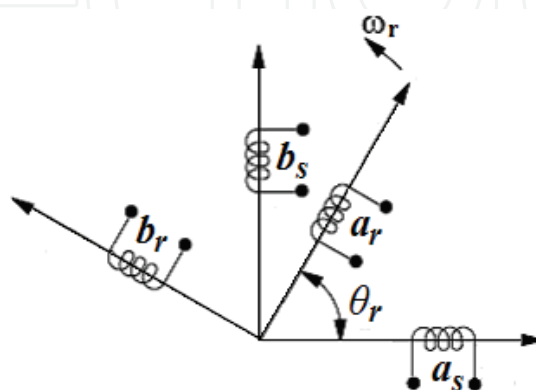
Fig. 1. Common reference frame ( a - b ).
