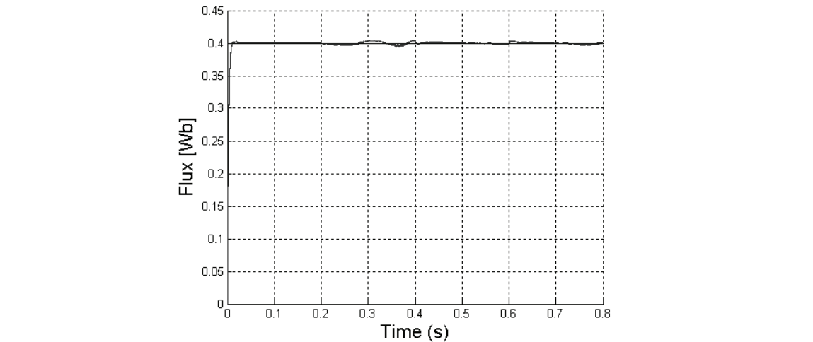
Fig. 10. Commanded and estimated flux
