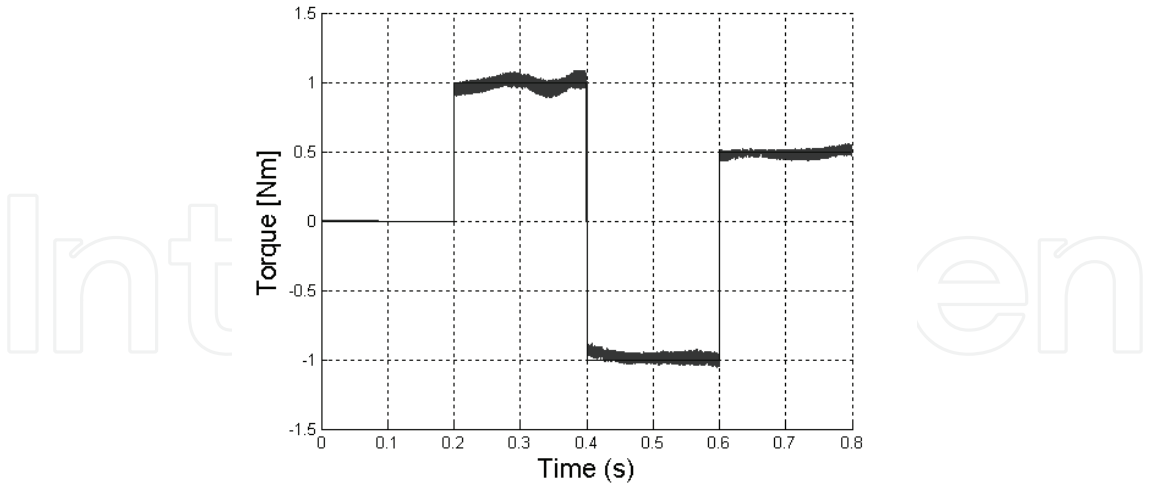
Fig. 9. Commanded and estimated torque (Nm).
