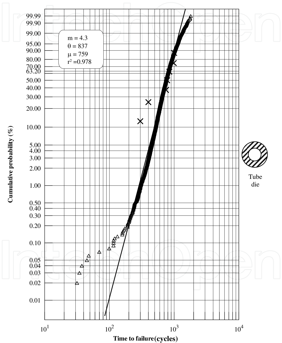
Fig. 6. Weibull model of fracture-failure simulation for the tube die
