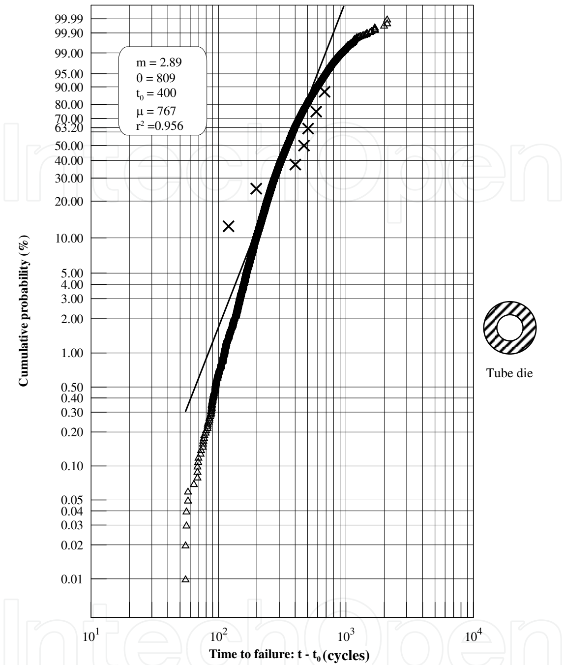
Fig. 10. Plot showing simulated wear life data and the fitted 3-parameter Weibull line for the tube die
