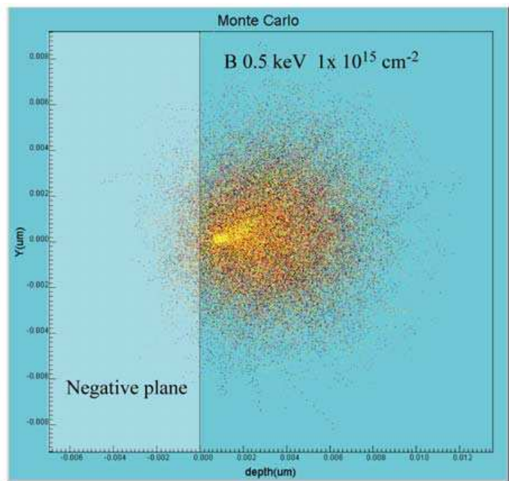
Fig. 12. MC tracing to the negative plane.
