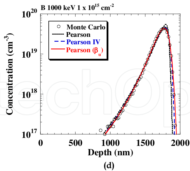
Fig. 15. MC simulation of B ion implantation profiles in Si substrates. Pearson function using raw moment parameters, and moment parameters of MC tracing to the negative plane are also shown The Pearson using the proposed B is also shown. (a) 0.5 keV, (b) 80 keV, (c) 160 keV, and (d) 1000 keV.
