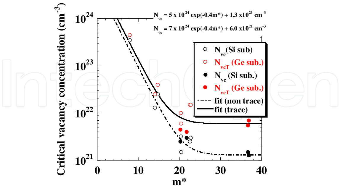
Fig. 26. Dependence of critical vacancy concentration on reduced mass. We hope to predict d_a for an unknown incident ion and substrate system. Fig. 26 shows the dependence of critical vacancy concentration on reduced mass. Any point is almost on lines of
