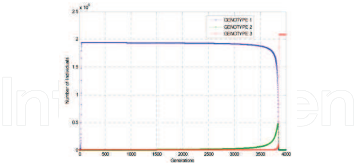
Fig. 1. Graphs of the Trajectories for the Three Genotypes as Computed by the Deterministic Model for the Female Population
