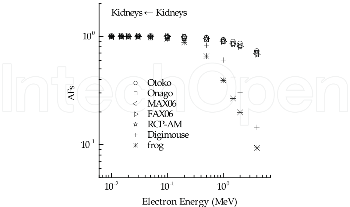
Fig. 4. Self-irradiation AFs in the Kidneys for the Otoko, Onago, MAX06, FAX06, RCP-AM, Digimouse and frog voxel models in the electron energy 10keV-4MeV.
