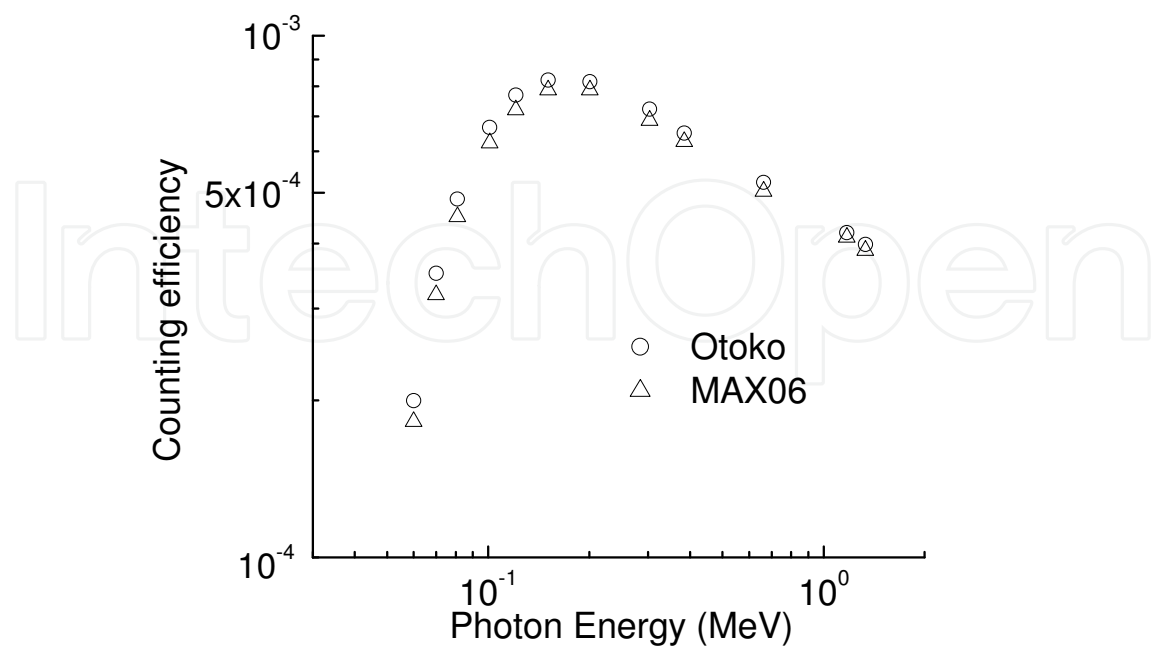
Fig. 7. Comparison of the counting efficiencies for the Otoko voxel model and those for the MAX06 voxel model.
