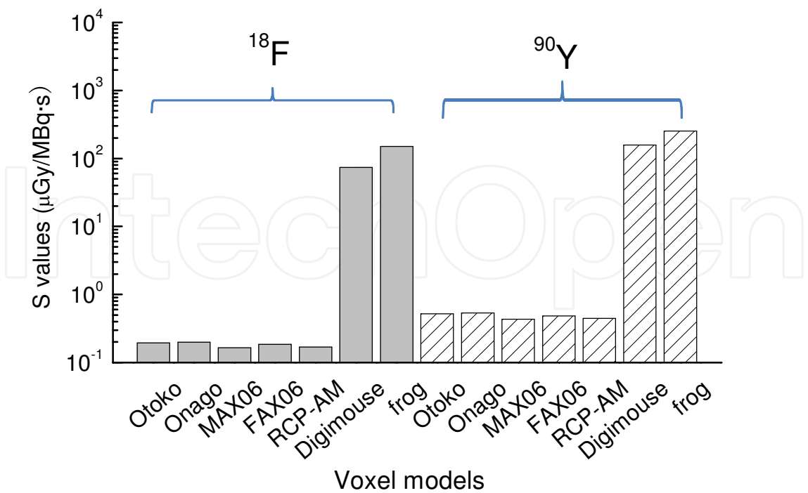
Fig. 6. Self-irradiation S values for 18 F and 90 Y in the kidneys of the Otoko, Onago, MAX06, FAX06, RCP-AM, Digimouse and frog voxel models.
