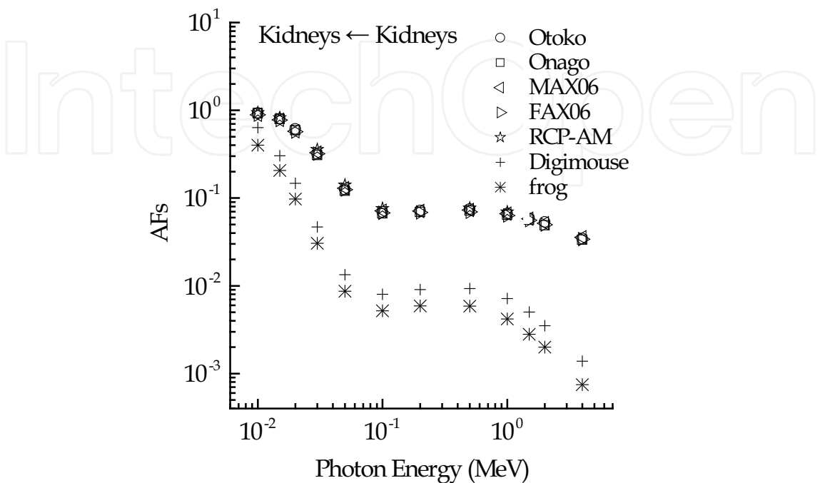
Fig. 3. Self-irradiation AFs for the >Kidneys in the Otoko, Onago, MAX06, FAX06, RCP-AM, Digimouse and frog voxel models in the photon energy 10keV-4MeV.
