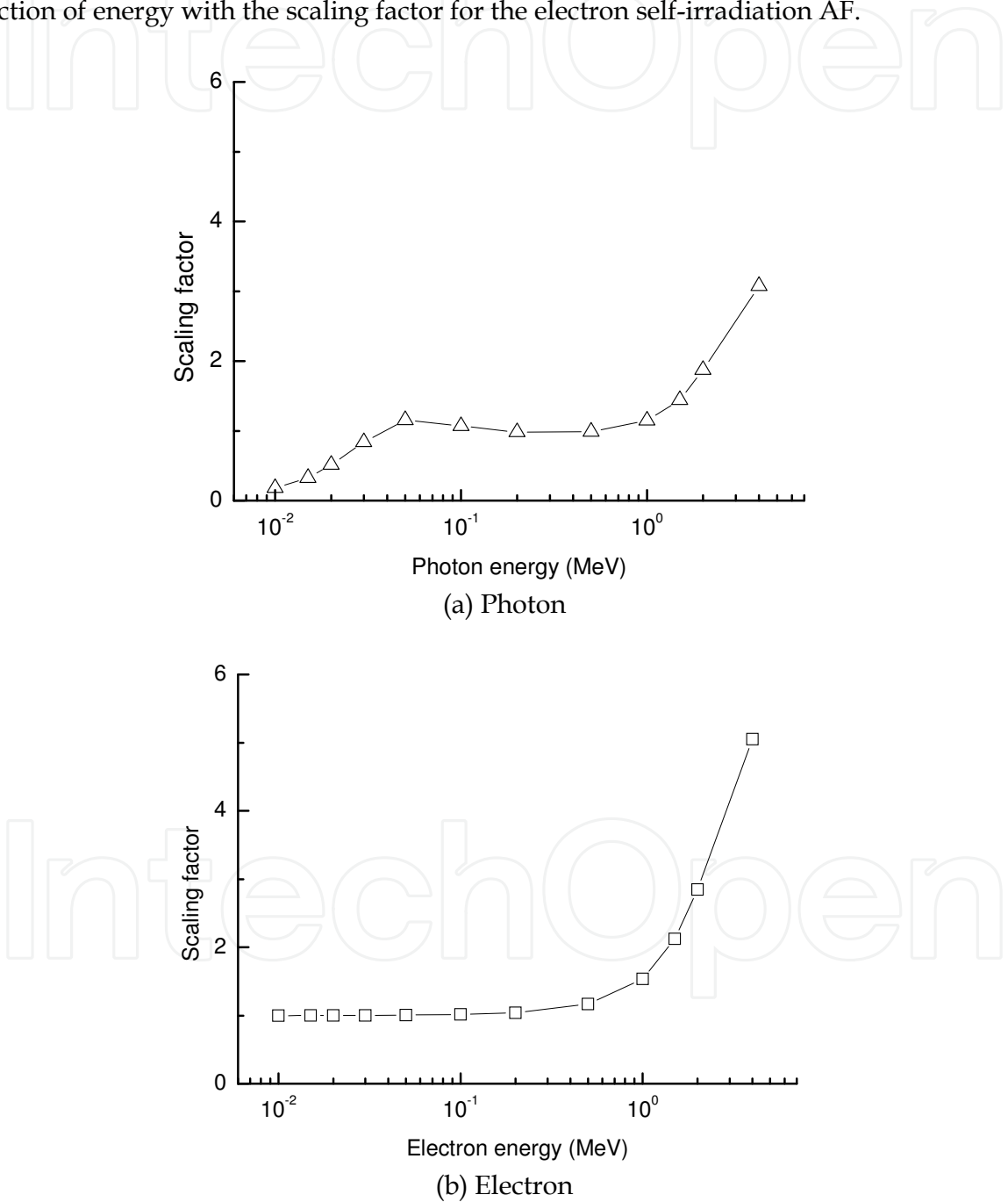
Fig. 5. Interspecies scaling factors of self-irradiation doses for the kidneys from the Digimouse voxel model to the Otoko voxel model in the energy 10keV-4MeV. (a) Photon, (b) Electron.
