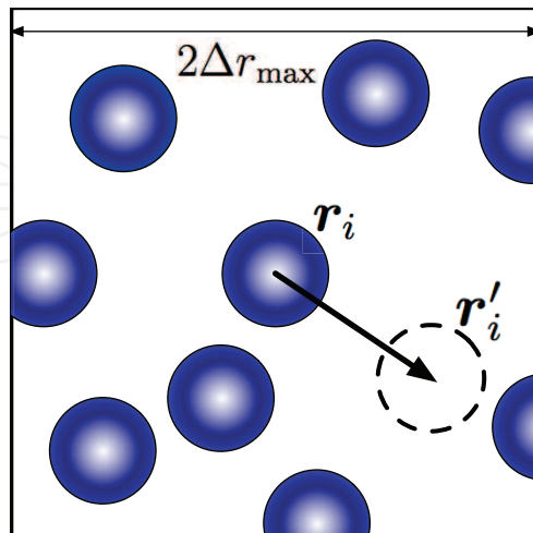
Fig. 3. Trial movement of particle i from position \mathbf{r}_i to \mathbf{r}'_i that can be any point within the square domain \mathcal{R} of each side 2\Delta r_{\max} .
