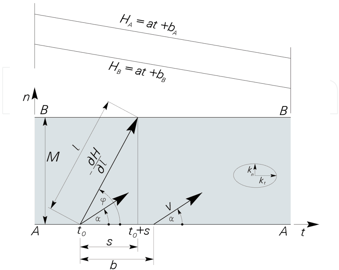
Fig. 1. Diagram of a flow through a single anisotropic layer. Let us accept that the flow occurs according to Darcy's law. Let us designate the hydraulic conductivity in a plane tangential to the aquifer floor and roof as k_t , and in the direction normal to that plane as k_n . Let the hydraulic head change linearly along line A-A (axis t ) according to the equation
