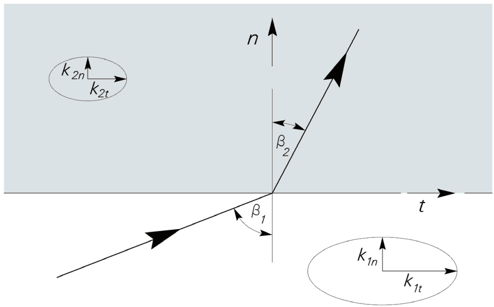
Fig. 2. Streamline refraction at the boundary of anisotropic layers. But
