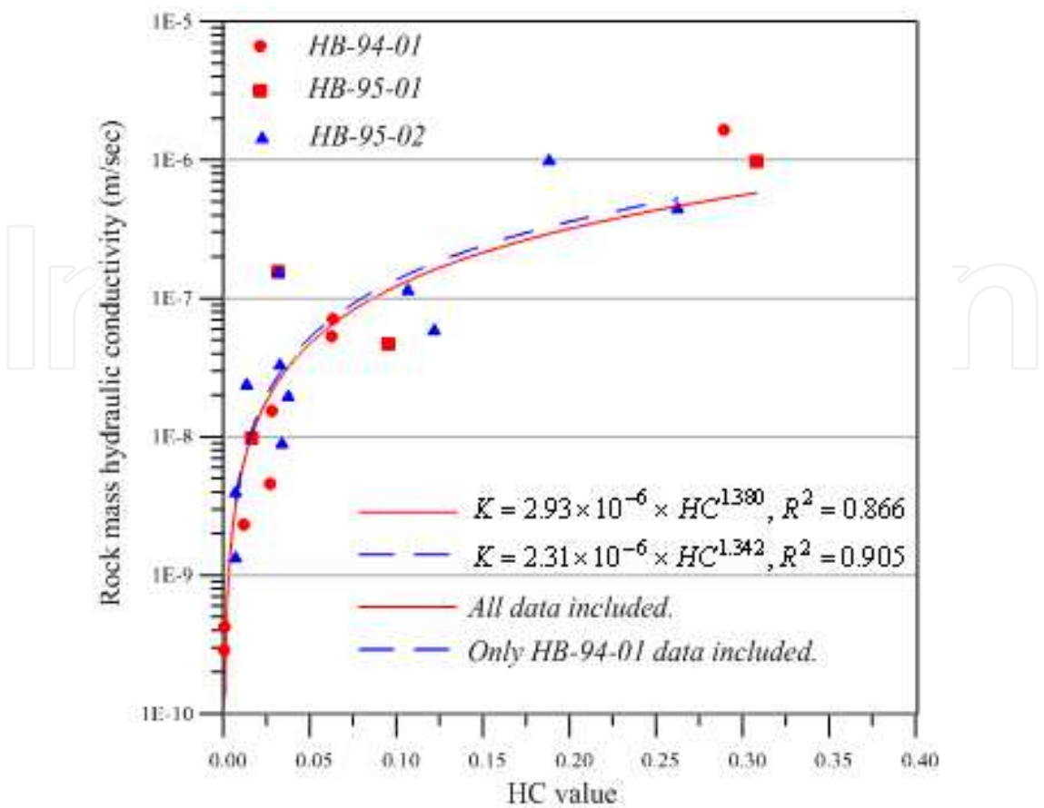
Fig. 6. Relationship between hydraulic conductivity and HC values
