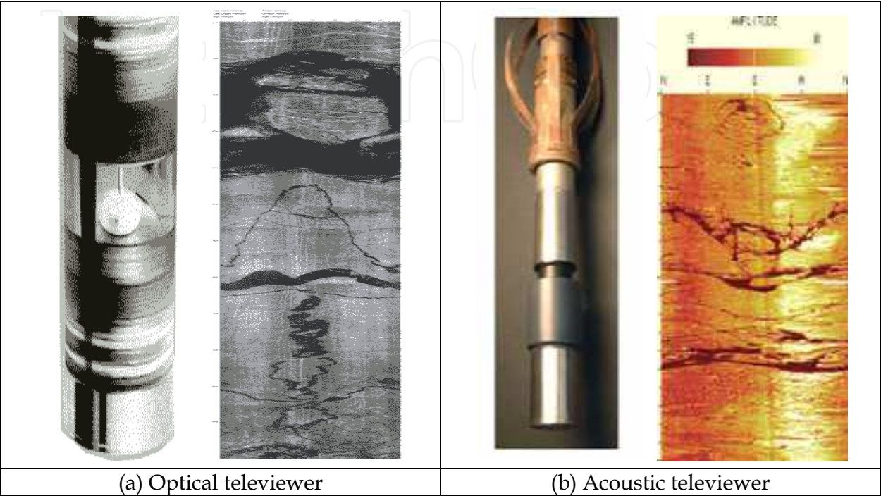
Fig. 8. The televiewer and scanned borhole images
