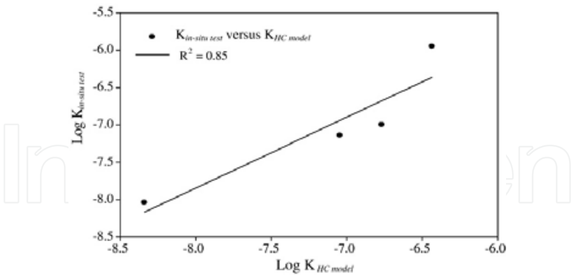
Fig. 7. Correlation between K HC-model and K in-situ
