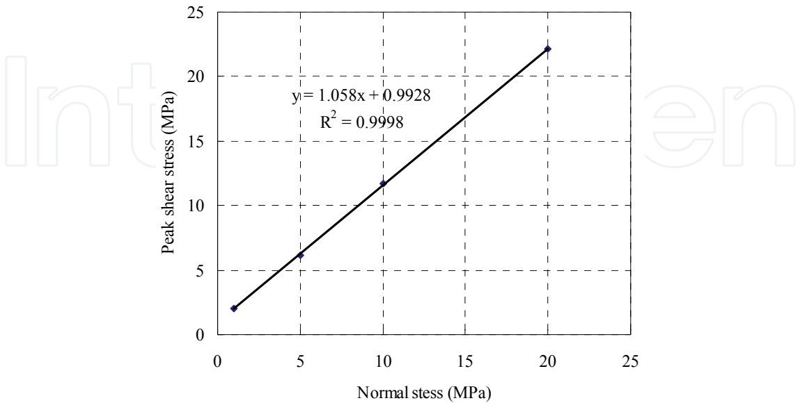
Fig. 8. Peak shear stress versus normal stress curve of the fracture.
