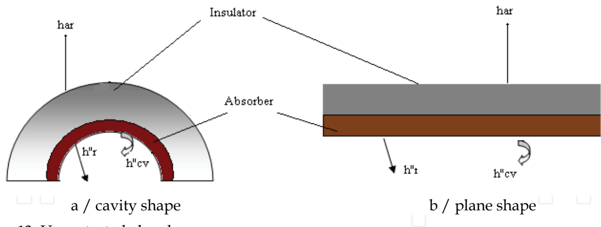
Fig. 13. Unprotected absorber.
