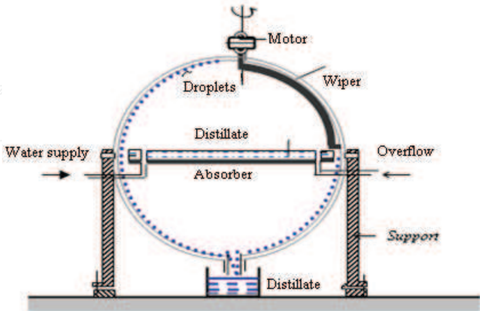
Fig. 3. Spherical solar distiller with sweeping
