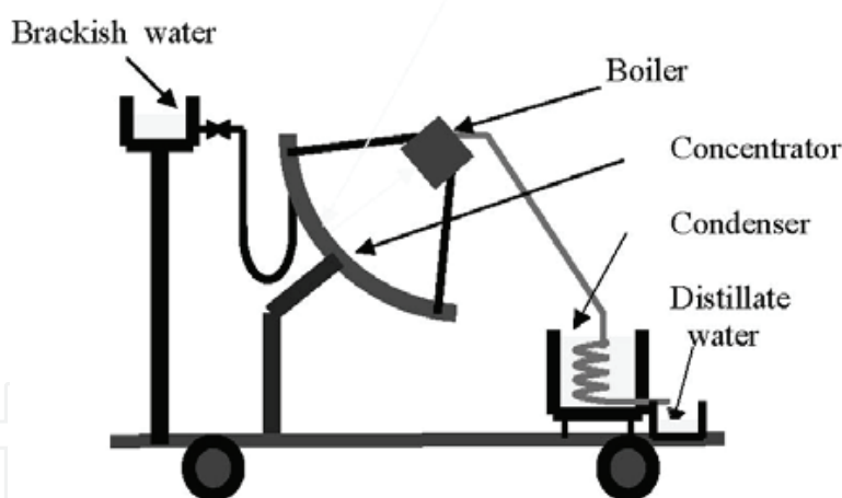
Fig. 15. Experimental device.
