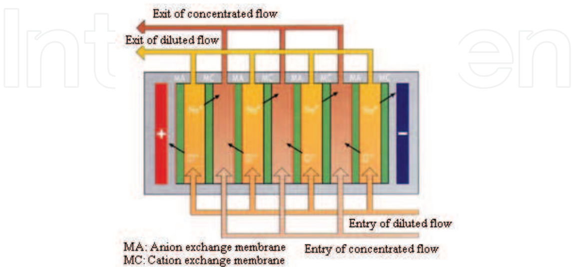
Fig. 8. Electrodialysis desalination process
