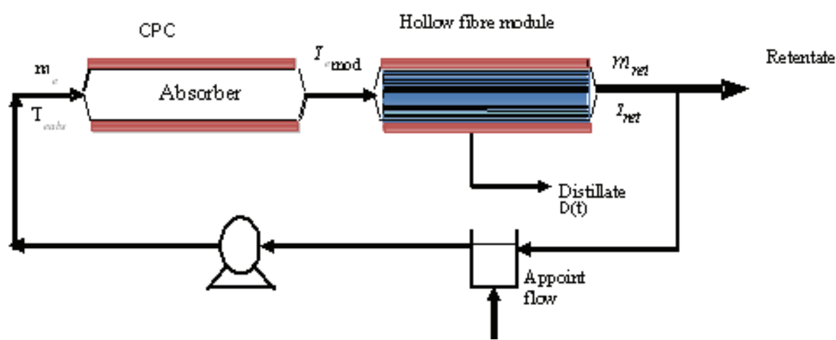
Fig. 10. Diagram of the desalination unit
