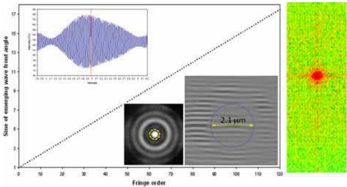
Fig. 8. System of fringes observed in the image of the 6 μm diameter polystyrene sphere. The dotted circle represents the first dark ring in the particle diffraction pattern
