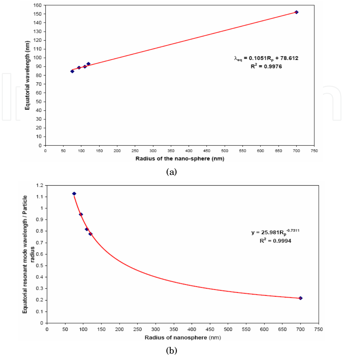
Fig. 19. Relationships between nanosphere radius and a) equatorial wavelength of the WG mode; b) normalized equatorial wavelength of the WG mode. was utilized in this study as the resonance modes occur approximately at the same wavelength, \lambda=386 nm. Figure 19a shows the equatorial wave length of the WG plotted vs. the particle radius. The experimentally measured wavelengths are plotted in a graph that includes also the numerically computed value (radius of 700 nm). A very good correlation ( R^2=0.9976 ) was obtained showing that the edge detection gradient utilized yields values that are consistent with the numerically computed WG wavelengths. The graph shown in Fig. 19b – the ratio of equatorial wavelength to radius is plotted vs. the radius – seems to provide a correlation with a better sensitivity. The correlation was again good ( R^2=0.9994 ).
