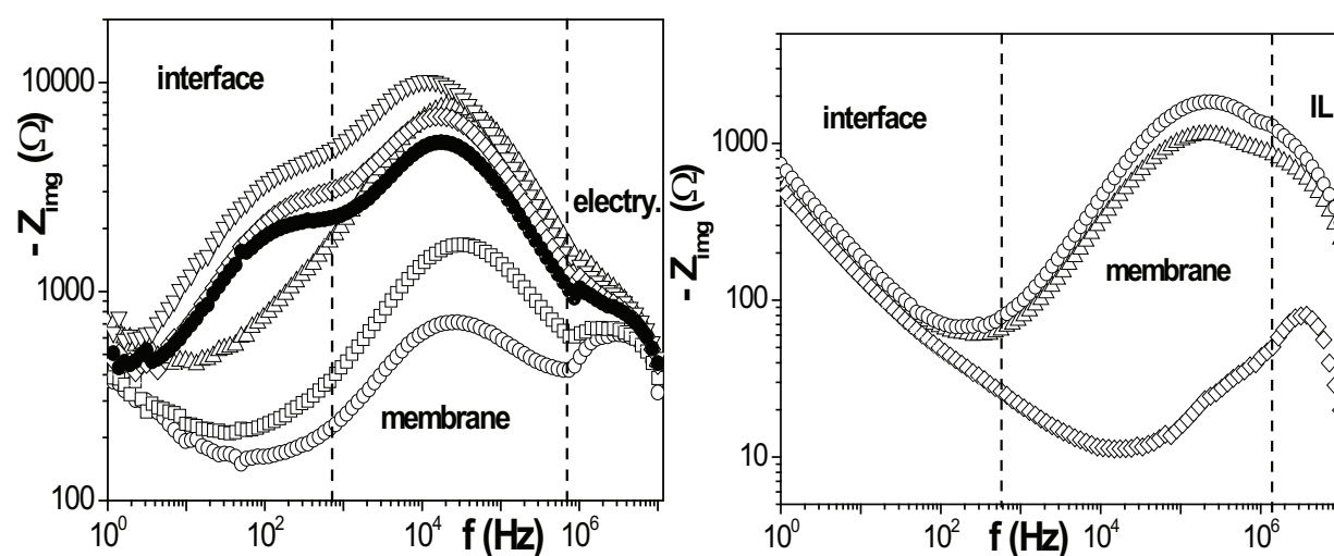
Fig. 10. (a) Time evolution of the Bode plot ( -Z_{\text{img}} vs frequency) for the Nafion membrane associated to IL-cation incorporation. (a) Nafion/DTA + system: (o) t = 0 , (□) t = 1 h, (Δ) t = 6 h, (▽) t = 19 h, (◇) t = 26 h, (●) t = 40 h. (b) Nafion/BMIM + system: (□) t = 1 h, (Δ) t = 5 h, (◇) t = 20 h.
