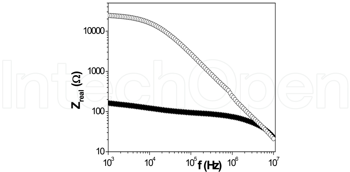
Fig. 12. A comparison of Z_{real} versus frequency plot for dry RC-6 ( \diamond ) and RC-6/BMIMBF 4 ( \blacklozenge ) membranes.
