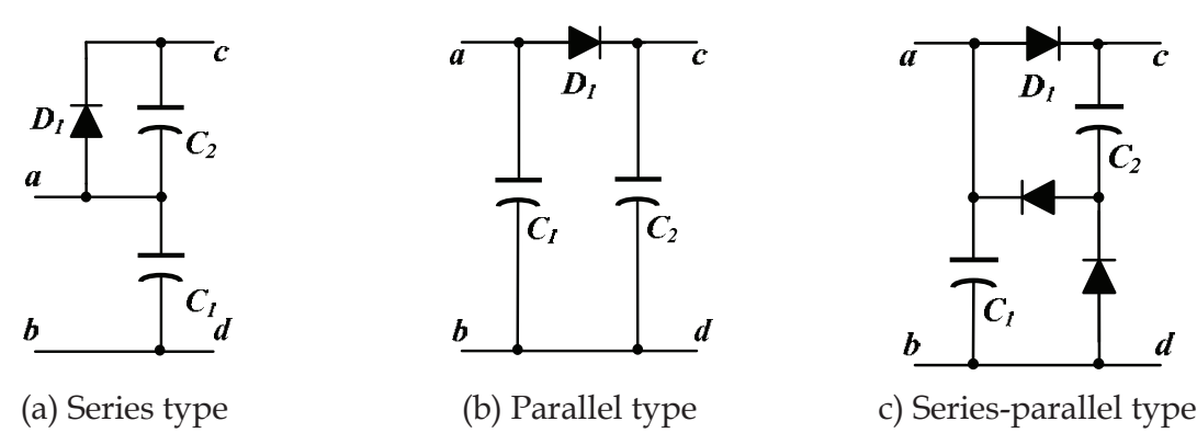
Fig. 19. Two capacitors network with diodes
