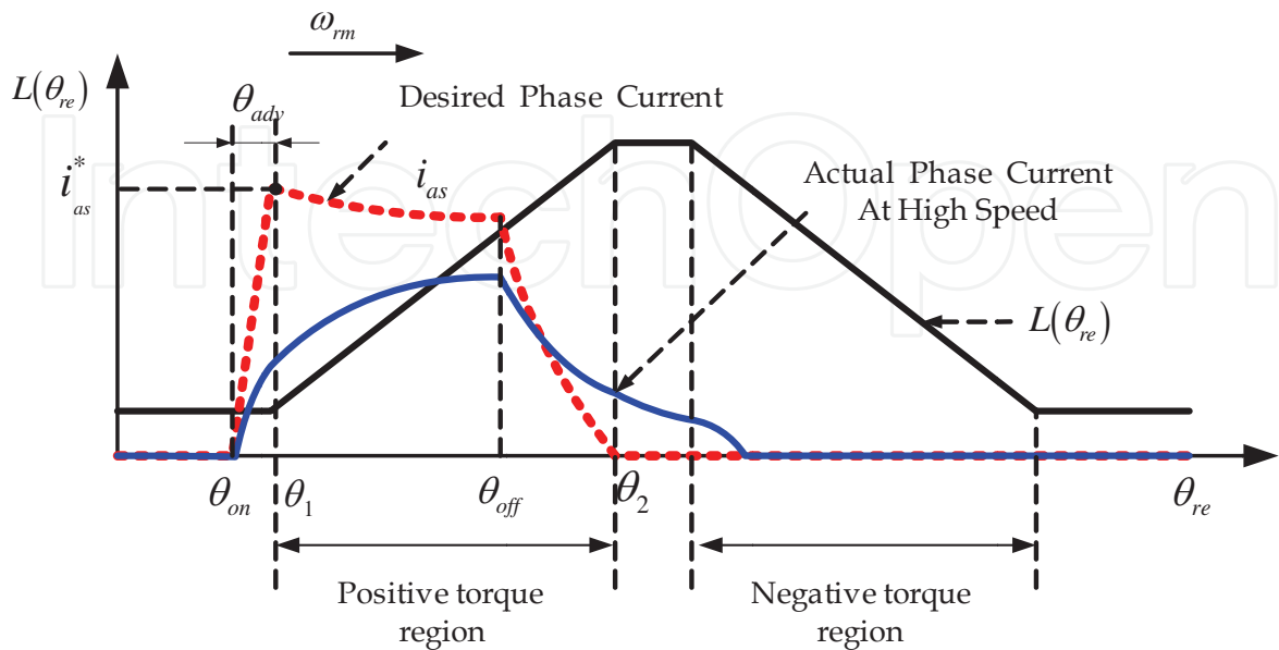
Fig. 40. Build-up of phase current in high speed region
