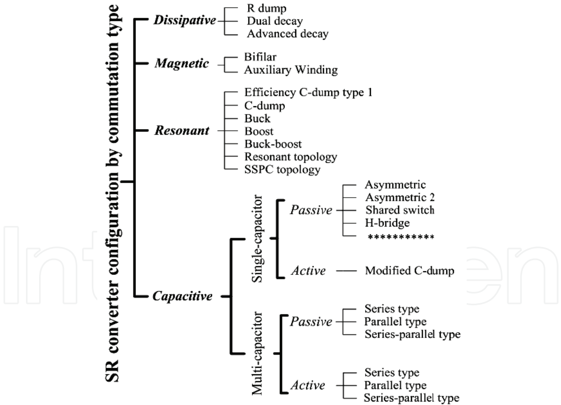
Fig. 24. SR converter configuration by commutation type
