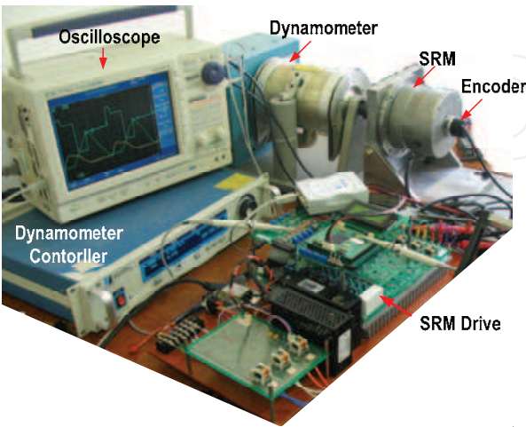
Fig. 61. The experimental configuration
