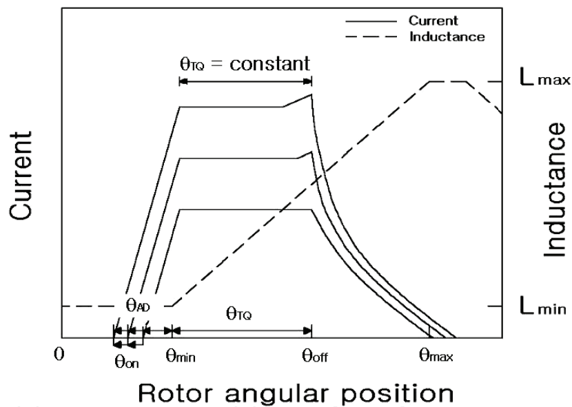
Fig. 38. Constant torque angle control
