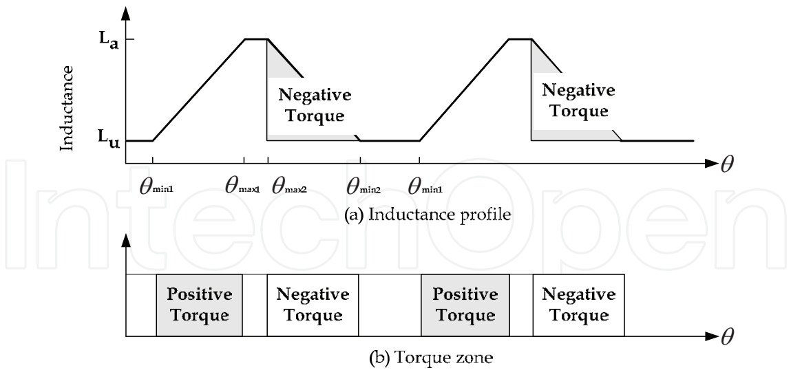
Fig. 8. (a)Inductance profile and (b) Torque zone
