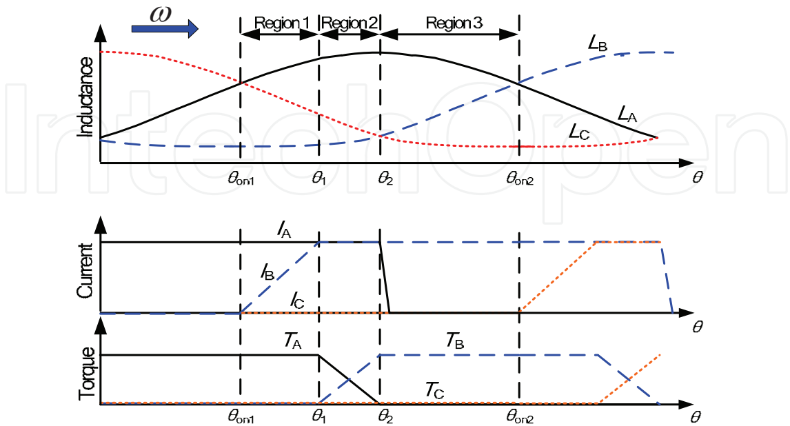
Fig. 47. Three regions of phase inductance in DITC method
