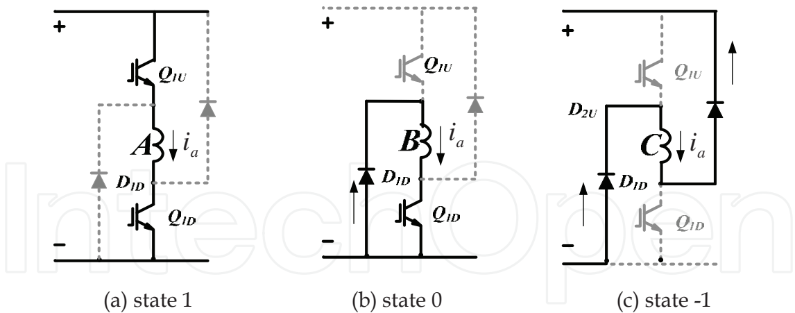
Fig. 46. 3 states in the asymmetric converter
