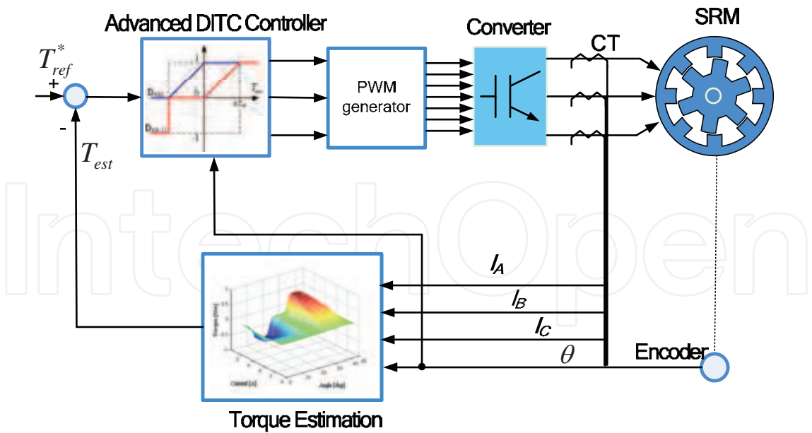
Fig. 53. Control diagram of ADITC
