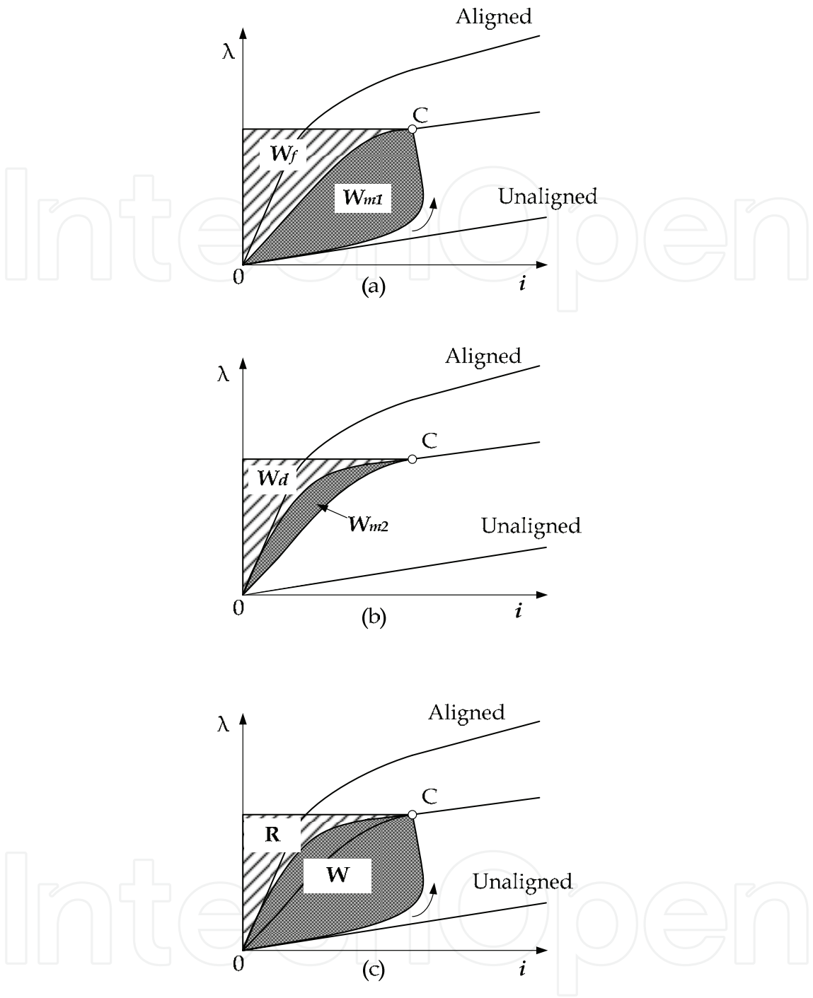
Fig. 11. Average torque (Energy conversion loop)
