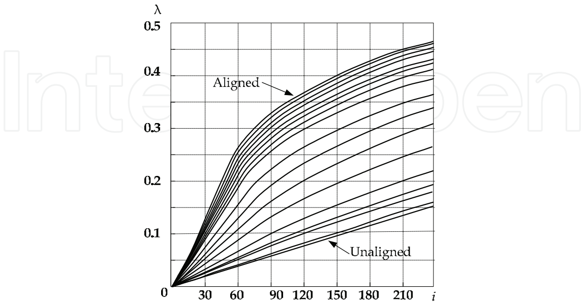
Fig. 9. Magnetizing curve and flux-linkage curve of SRM
