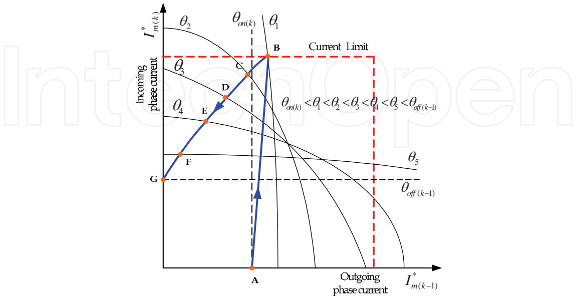
Fig. 58. The ideal current trajectory at commutation region
