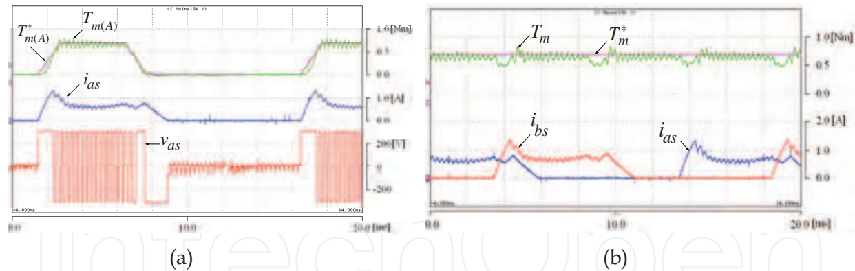
Fig. 62. Experimental results in linear TSF(at 500[rpm]) (a) Reference torque, actual torque, phase current and terminal voltage (b) Total reference torque, actual torque and phase currents
