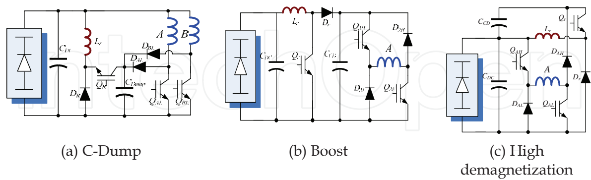
Fig. 27. Three types of resonant SR converter
