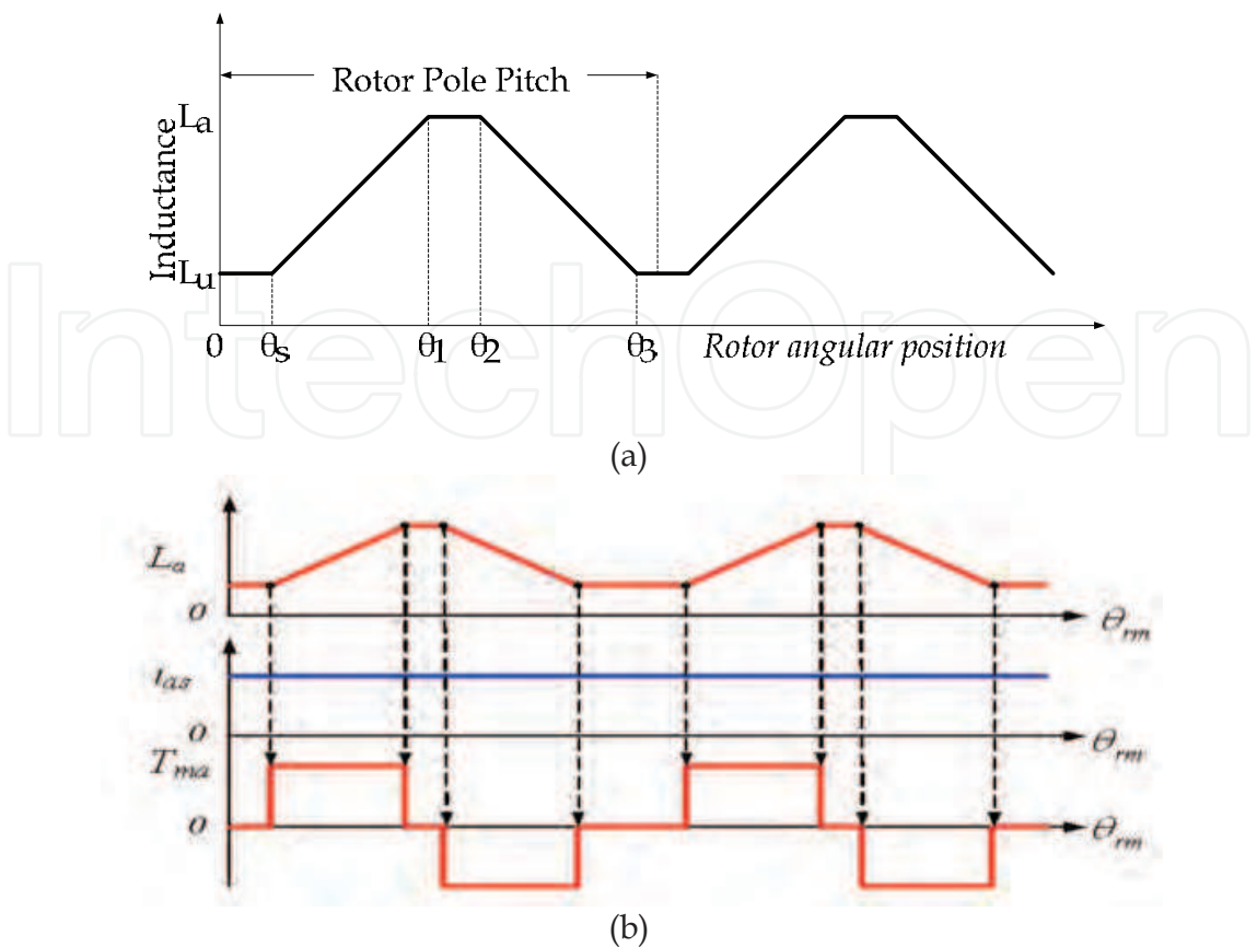
Fig. 2. (a) Inductance and (b) torque in SRM
