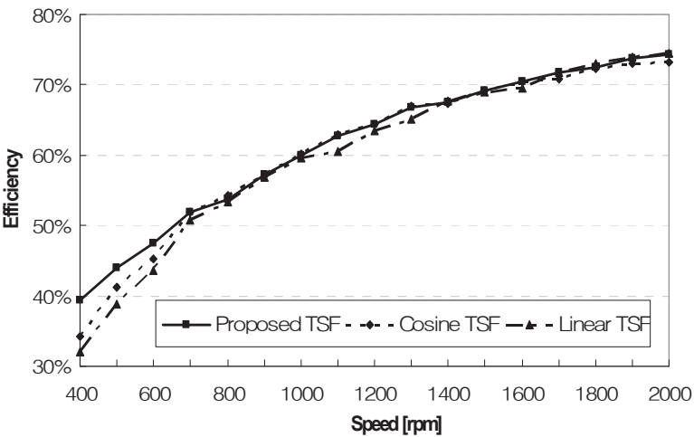
Fig. 66. Efficiency comparison
