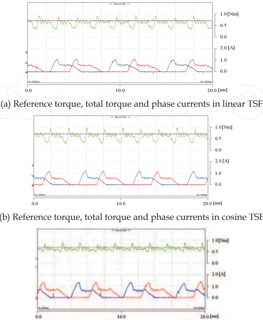
Fig. 65. Experimental results at 1200rpm with rated torque
