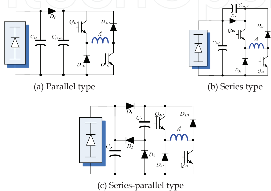
Fig. 30. Passive boost converter with two capacitors
