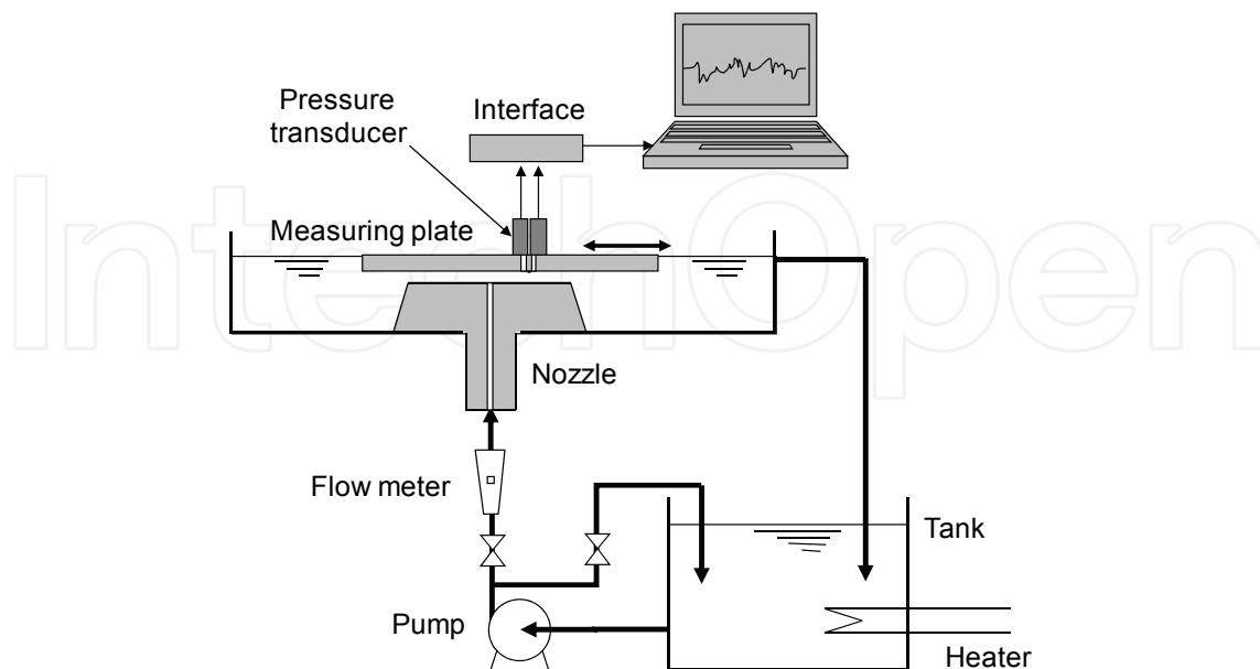
Fig. 11. Set-up for the system to measure the near-wall hydrodynamic conditions of a specimen in the jet-in-slit corrosion testing apparatus.
