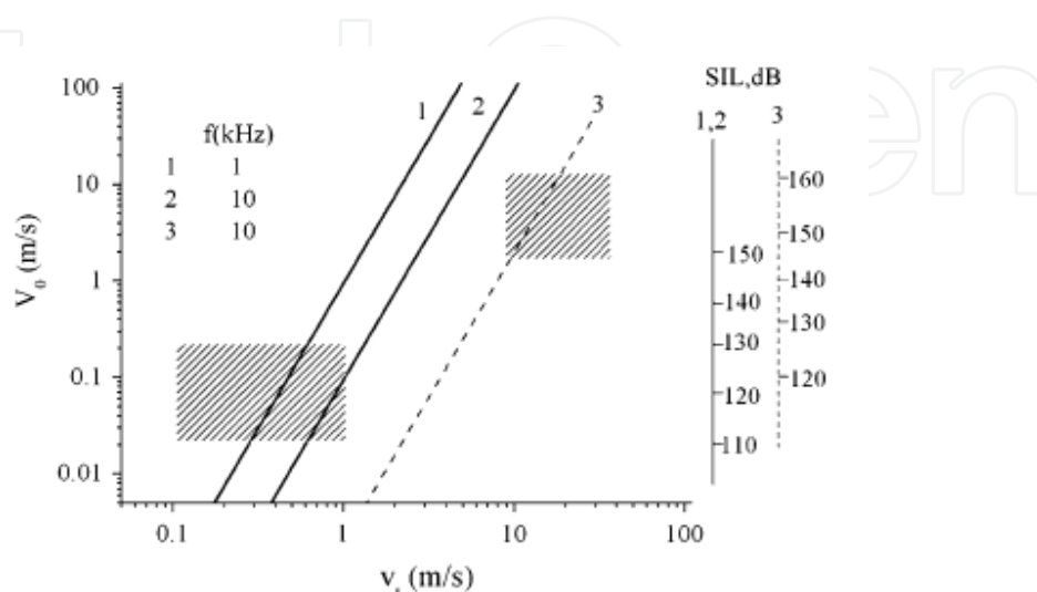
Fig. 8. A plot of V_0 versus v_t : 1 and 2 – cold model, 3 – pilot converter
