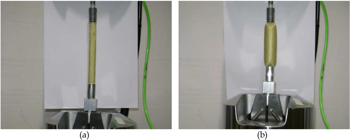
Fig. 3. Characterization testing of PAM actuator – (a) resting length; (b) free contraction contraction value and is shown in Figure 3(b). After recording this value, the PAM actuator was stretched back to its resting length and the test was stopped. Typical performance data from each of the three selected PAM configurations is provided in Figure 4 at various pressure settings. Note that the x-axis data is presented as the non-dimensional contraction percentage. For the range of PAM lengths considered in this work, it has been shown that contraction percentage is largely independent of PAM length for a given diameter and braid angle. As an example, a particular PAM at a given pressure may have a free contraction of 25%. This actuator with a 4-in resting length would thereby have a free contraction of 1 inch, whereas a 12-in resting length actuator would have a free contraction of 3 inches. It can be seen in Figure 4 that both force and contraction increase with pressure. For the performance metric of blocked force (measured force with 0% contraction, i.e., resting length and maximum possible force), the increase in force is linear with pressure, but the same is not true for the performance metric of free contraction (measured contraction with 0 lb force, i.e., maximum possible stroke). The free contraction increases with pressure, but tends to roll off as a maximum limit is approached. These trends are valid, of course, only over the pressure range which does not lead to yield in the braid fibres. It should be noted here that our tests have shown that the PET braid does not begin to yield until approximately 200 psi and the yield point for the Kevlar braid is over 1000 psi. Given that the three system designs here are all intended to operate below 100 psi, a more than adequate safety margin exists for burst failure. Another characteristic to mention in regard to the typical force-contraction
