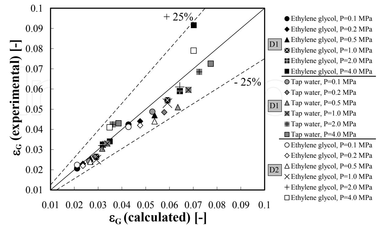
Fig. 5. Parity plot for gas holdups in ethylene glycol and tap water aerated with nitrogen through gas distributors D1 and D2 at various pressures
