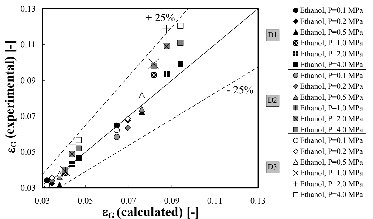
Fig. 6. Parity plot for gas holdups in ethanol (96 %) sparged with nitrogen through gas distributors D1–D3 at various pressures
