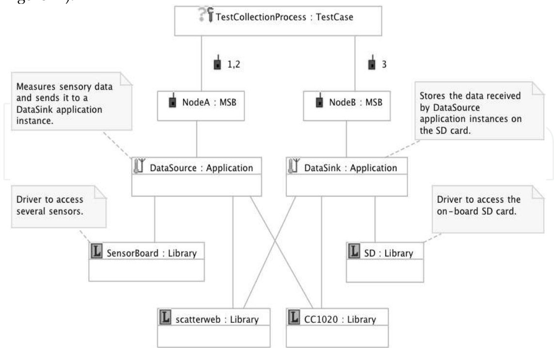
Fig. 14. Test case within an application
