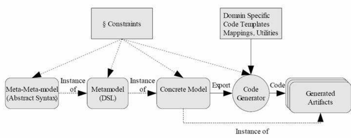
Fig. 2. AC-MDSD as product-line
