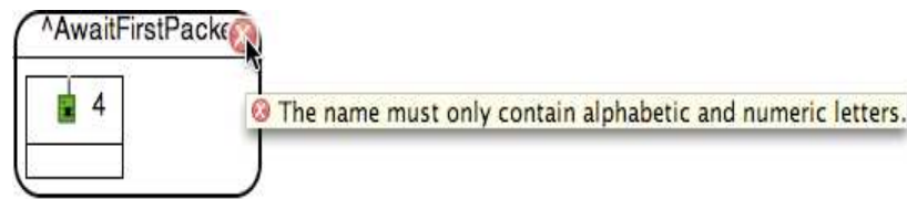
Fig. 11. Live-Validation detected an invalid name
