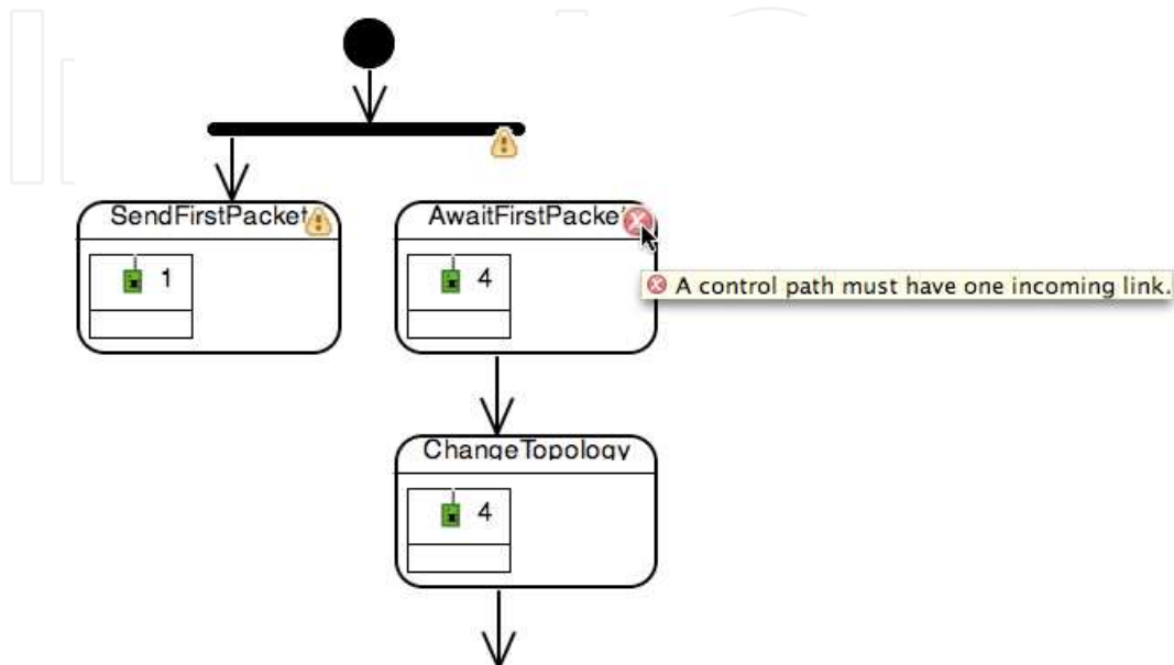
Fig. 12. Live-Validation detected a control path with no predecessor
