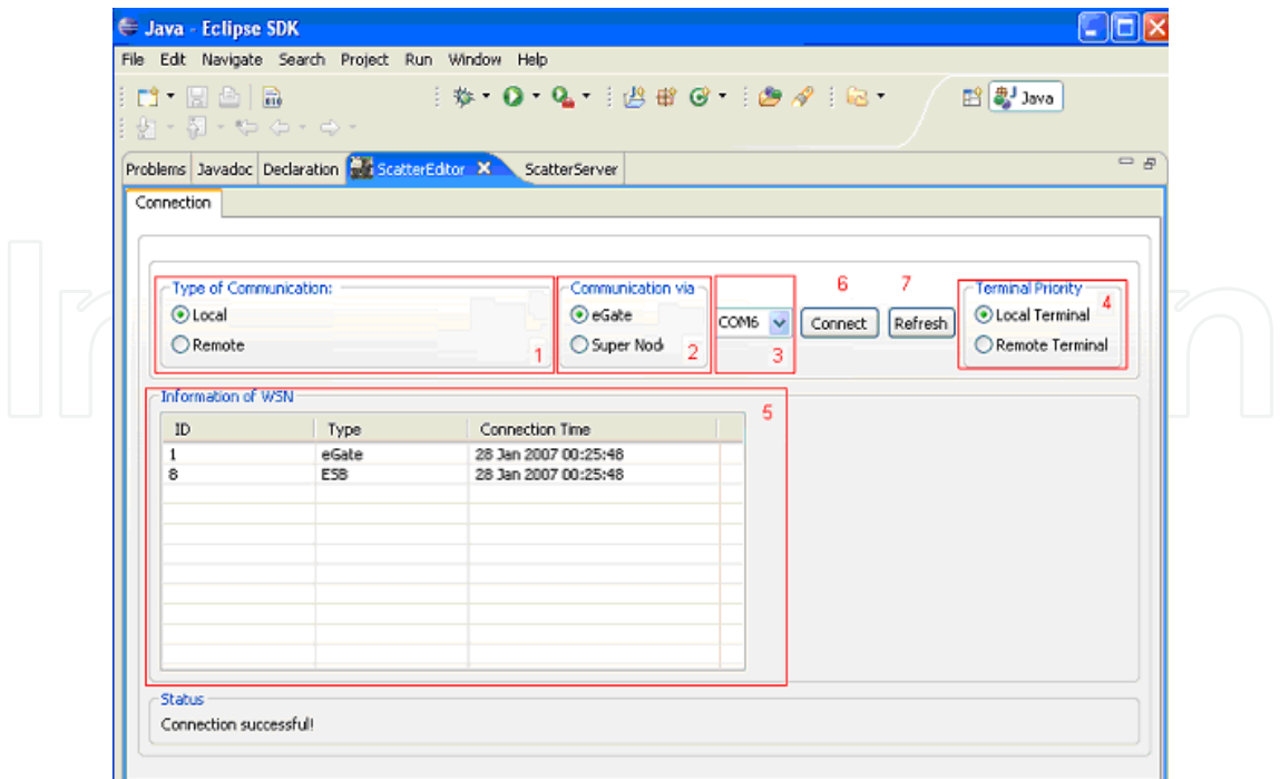
Fig. 15. Connection Tabfolder
