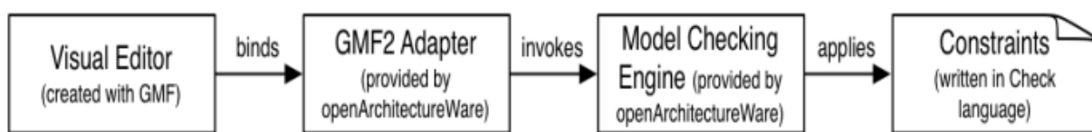
Fig. 10. Live-Validation Components
