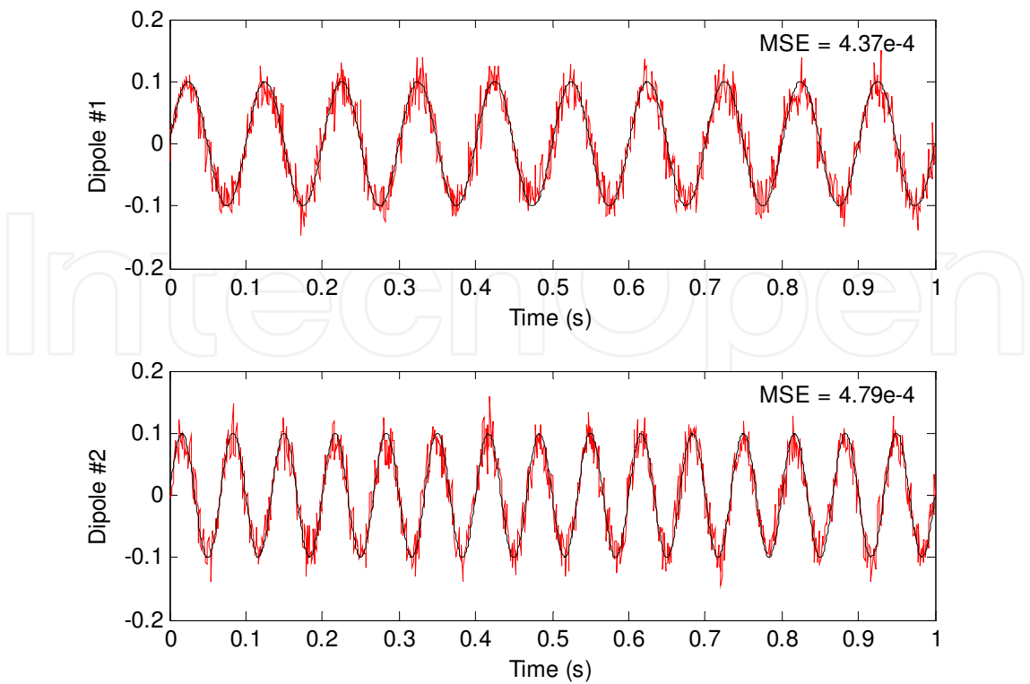
Fig. 2. The original and estimated source waveforms represented together for dipole 1 (top) and dipole 2 (bottom) using the LCMV beamformer
