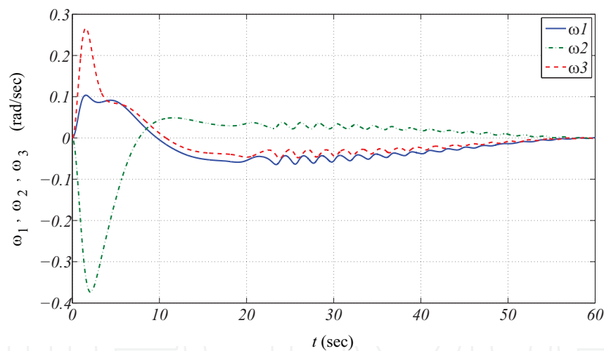
Fig. 3. Angular velocity components vs. Time: rest-to-rest slew maneuver
