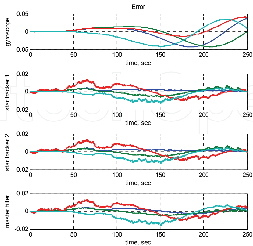
Fig. 5. Error between true quaternion and estimates (normal condition)
