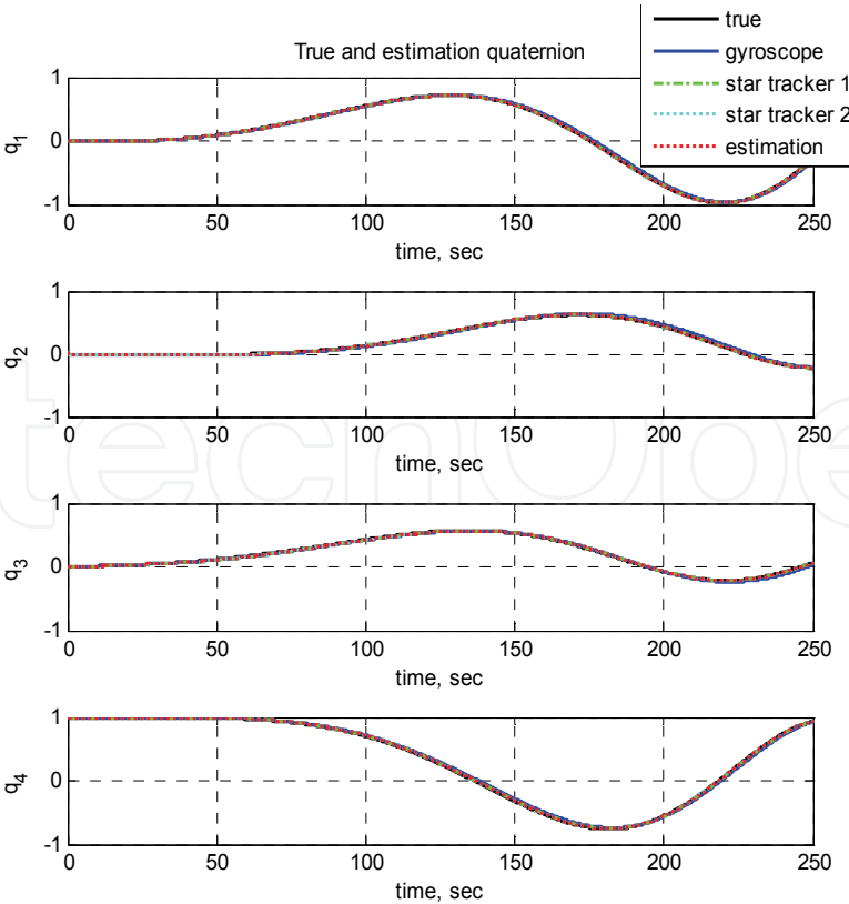
Fig. 4. Local and global estimates (normal condition)
