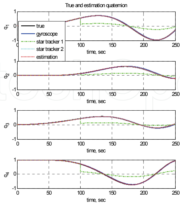
Fig. 15. Local and global estimates with FDI algorithm (star tracker fault)
