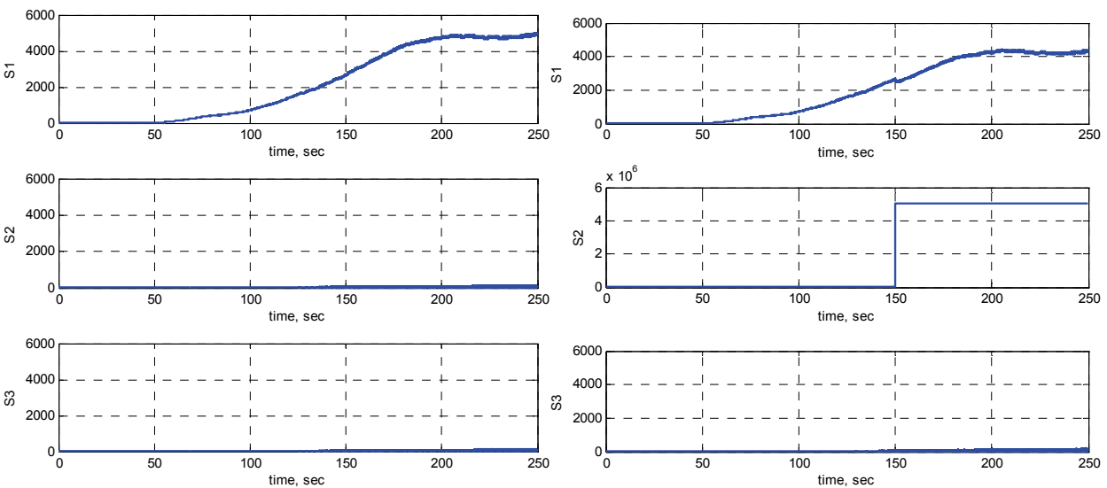
Fig. 2. Time histories of sensitivity factor: (a) normal case (left), (b) failure case (right)
