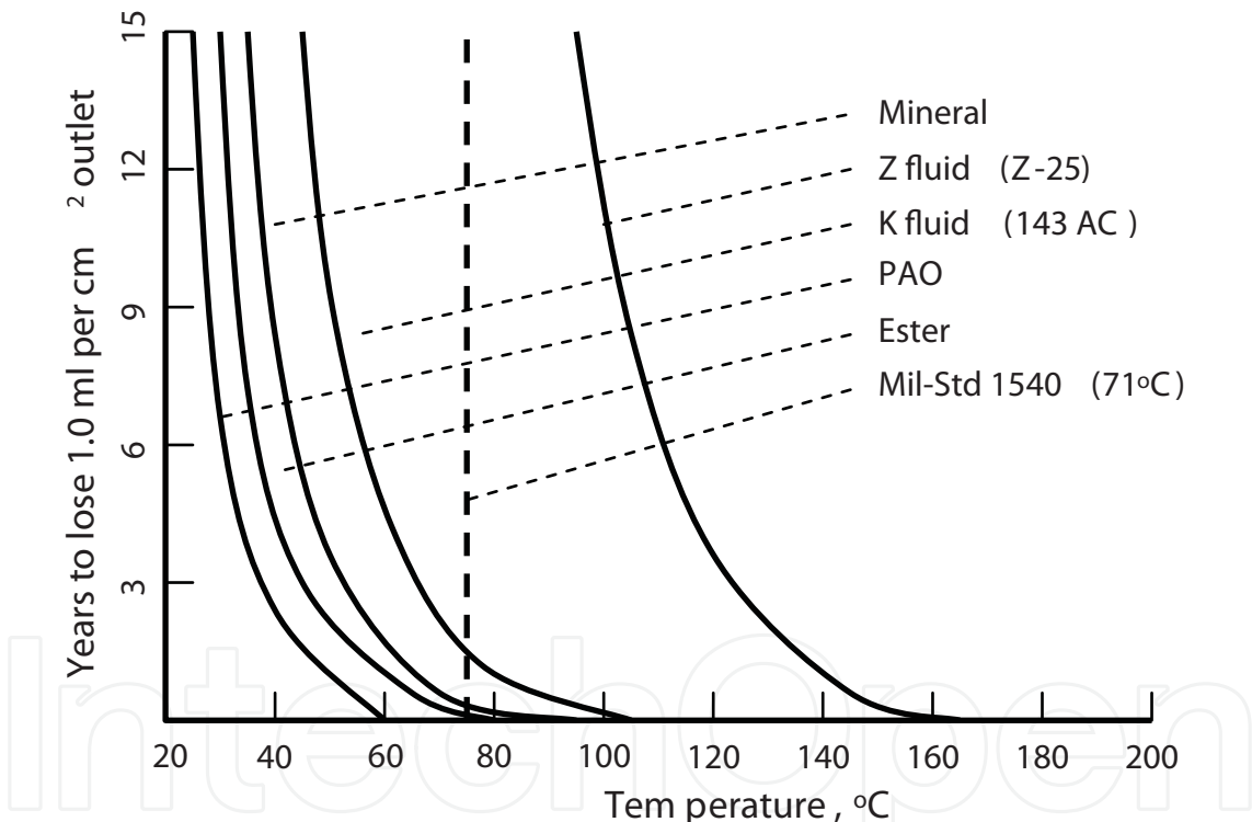
Fig. 6. Evaporation rates of various aerospace liquid lubricants (Jones and Jansen, 2005)
