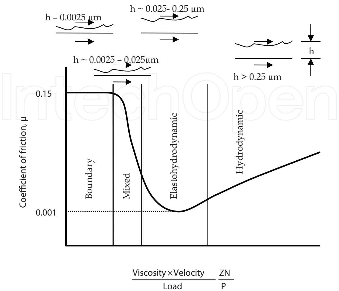
Fig. 4. Stribeck/Hersey curve (Fusaro, 2001)
