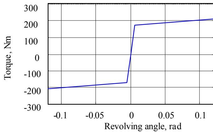
Fig. 9. Torque and angle in roll
