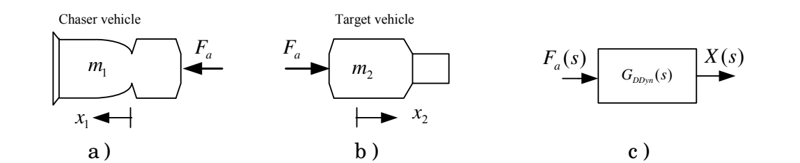
Fig. 18. Single-DOF spacecraft bodies Above dynamics model is also a simplified version of the dynamics model actual spacecraft bodies shown in Figure 5. The docking mechanism of the single DOF can be simplified as a spring and a damper, shown in Figure 19. Its mathematic model of the docking mechanism can be written as
