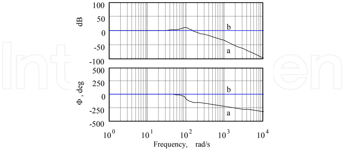
Fig. 23. Bode diagram of simulation/ hardware interface
