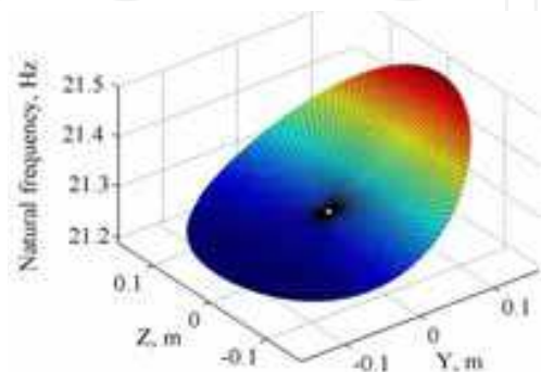
Fig. 32. Natural frequency in Y direction
