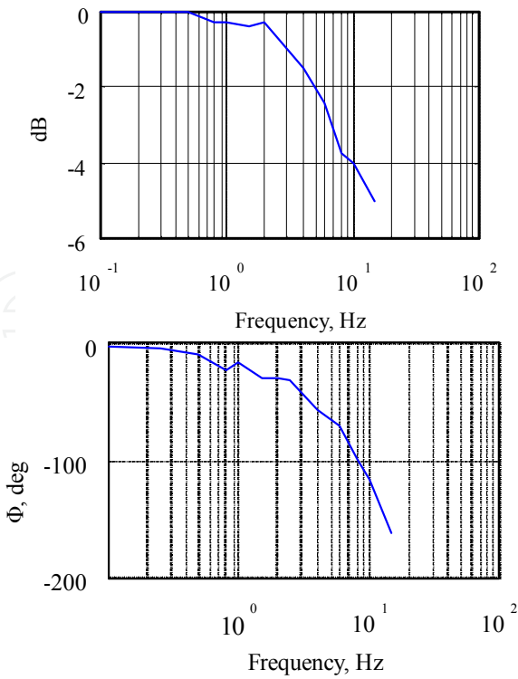
Fig. 40. Bode diagram in Y direction
