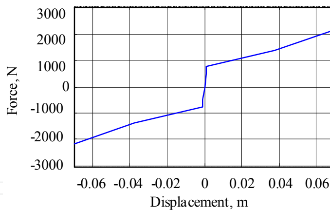
Fig. 7. Force and displacement Y or Z direction
