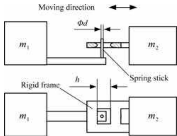
Fig. 37. Vibro-impact HIL simulation test
