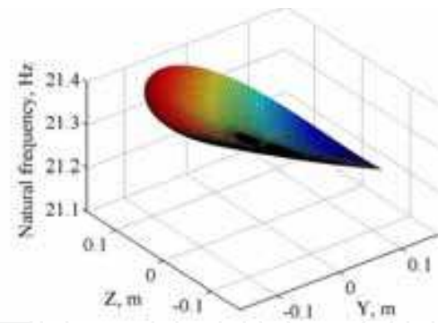
Fig. 33. Natural frequency in Z direction
