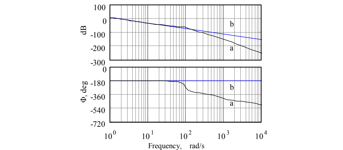
Fig. 24. Bode diagram of HIL simulation system
