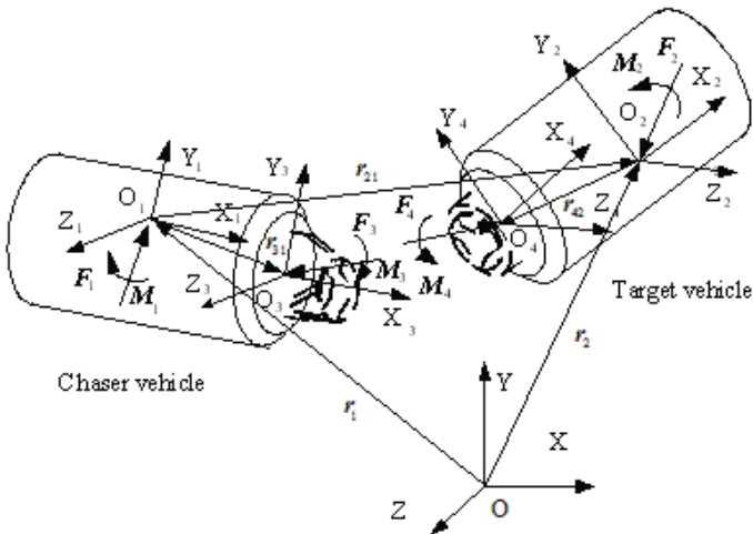
Fig. 2. On-orbit docking spacecraft bodies
